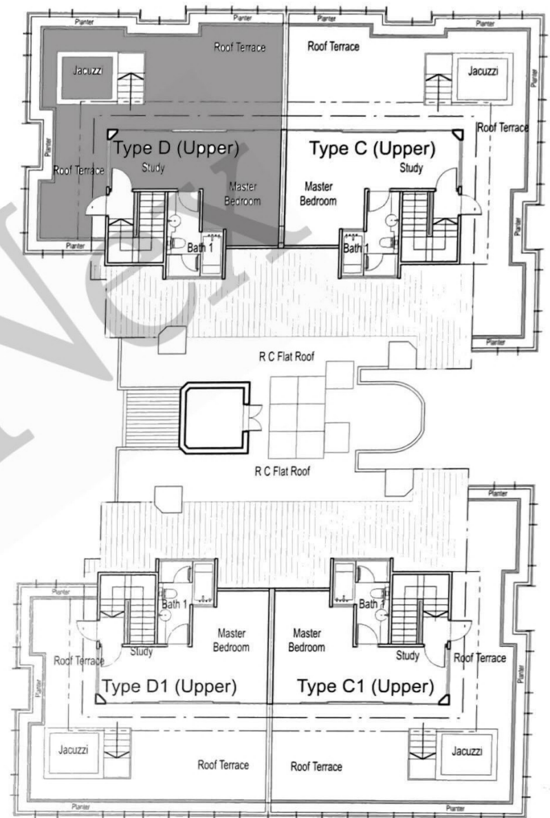
Attic Plan
