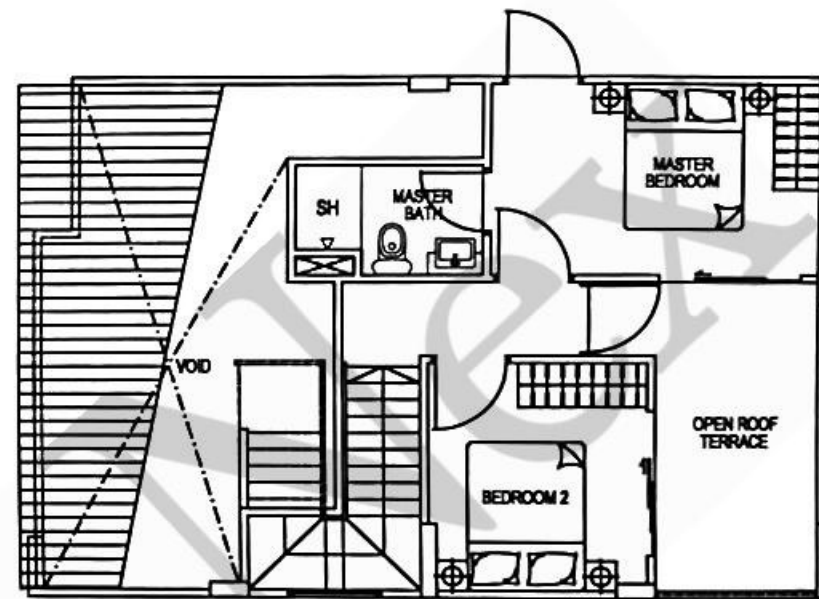
UPPER STOREY
