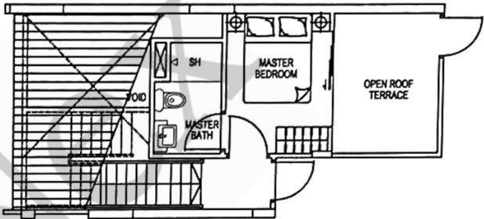
UPPER STOREY
