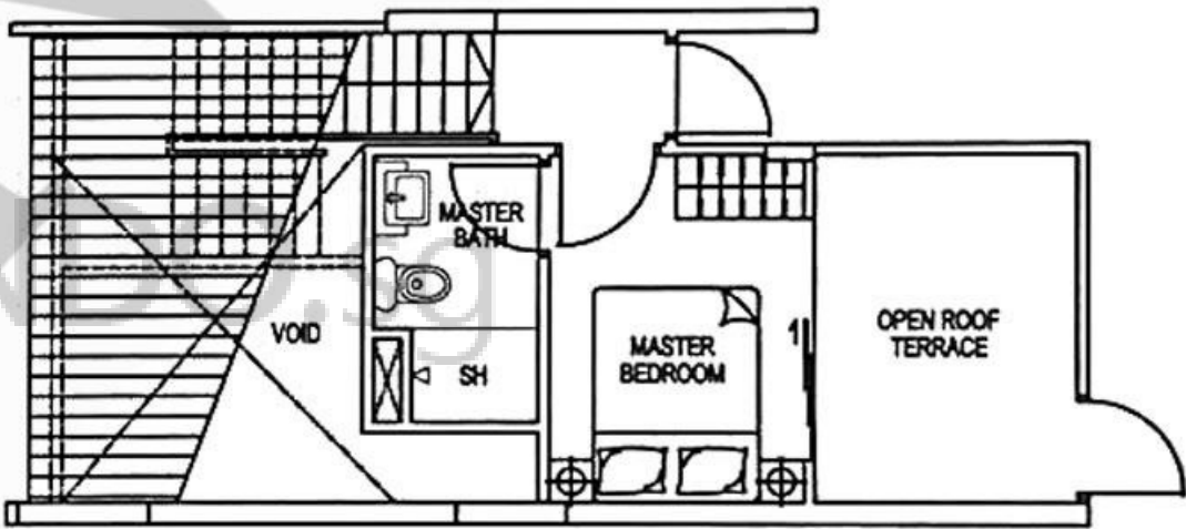
UPPER STOREY
