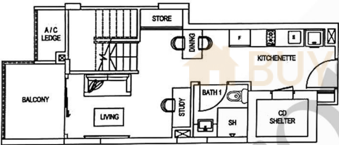
LOWER STOREY
