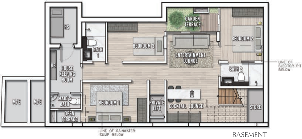
BASEMENT
