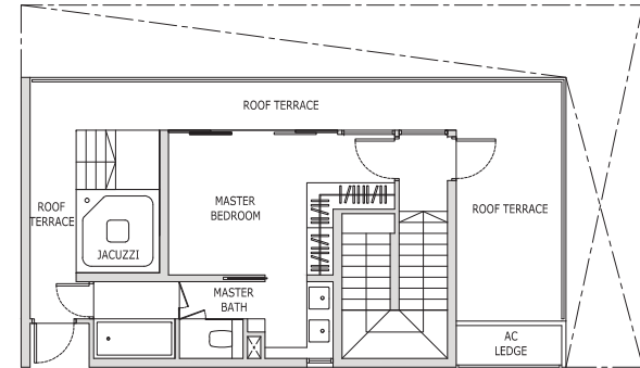
Upper Level
