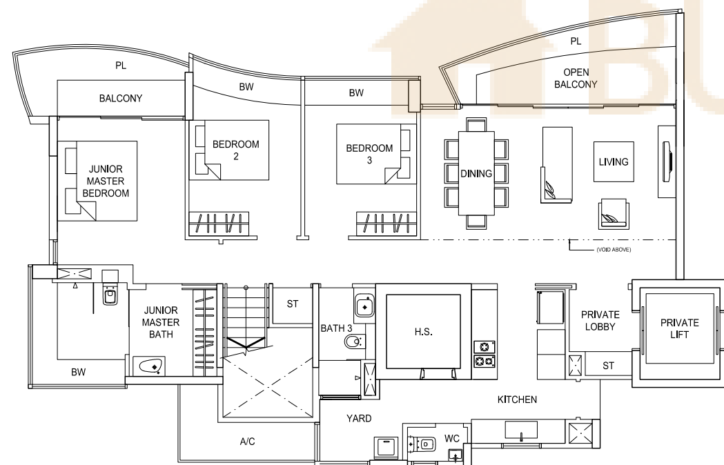
TYPE PH2(Lower Level)
