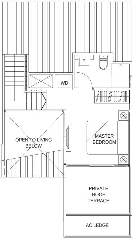
UPPER LEVEL
