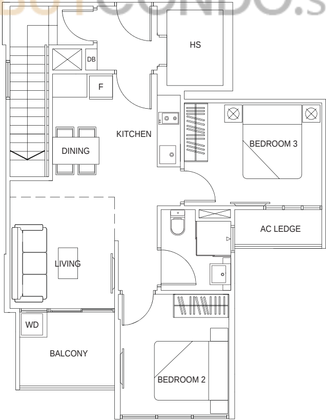
LOWER LEVEL
