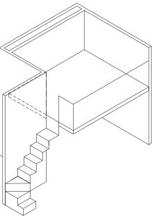
LOFT ISOMETRIC VIEW
