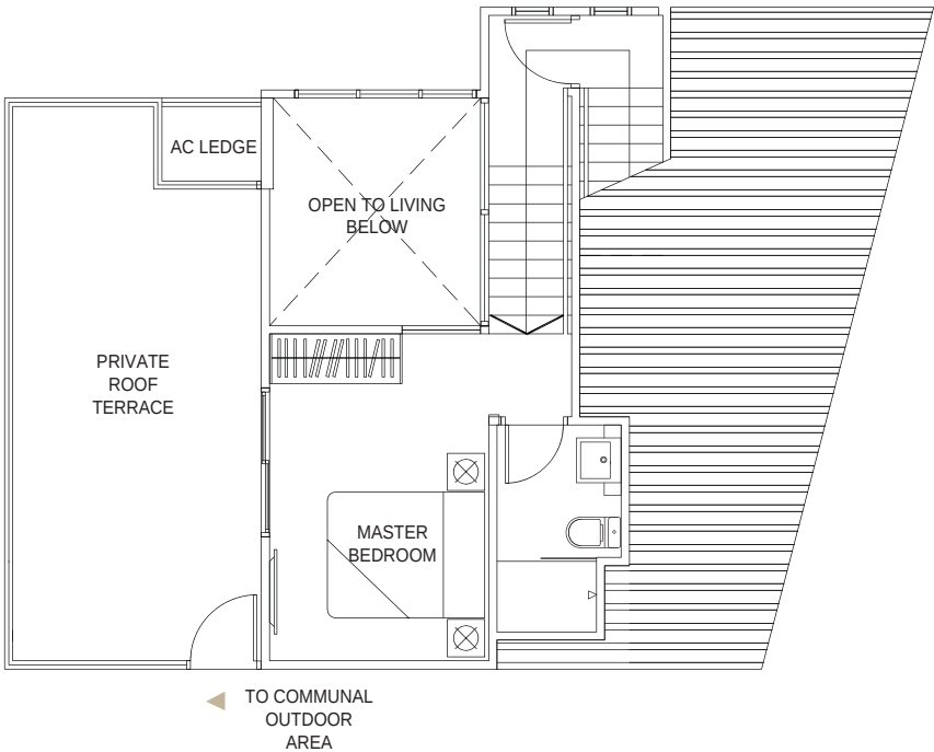
UPPER LEVEL
