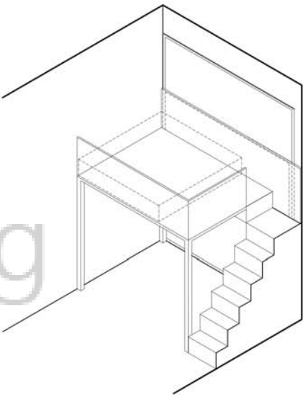
SUGGESTED LOFT LAYOUT ISOMETRIC VIEW
