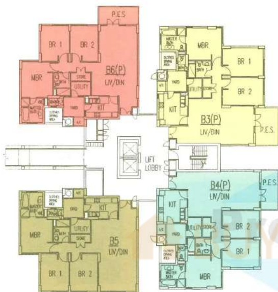
31 Bangkit Rd 1st Storey Plan
