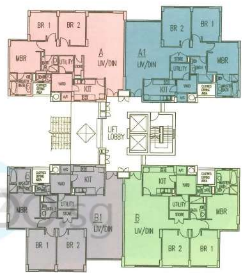
33 Bangkit Rd 2nd - 4th Storey Plan
