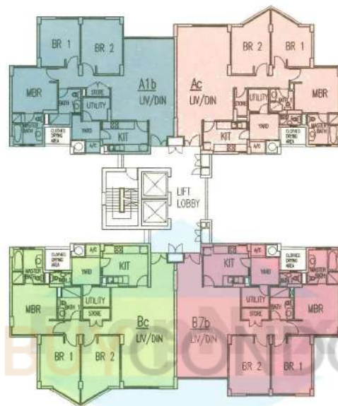
35 Bangkit Rd 17th Storey Plan
