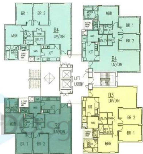
41 Bangkit Rd 2nd - 4th Storey Plan
