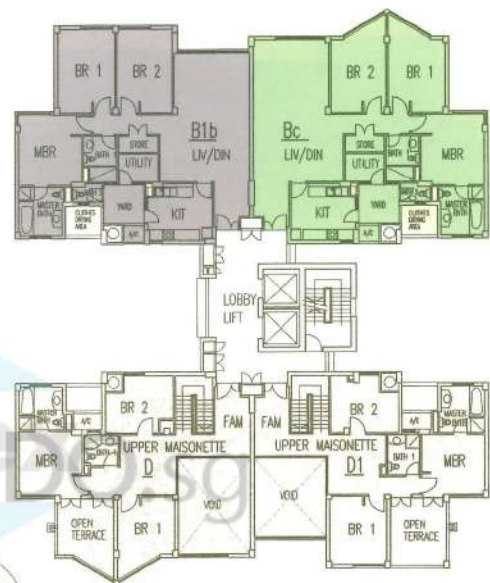
39 Bangkit Rd 15th Storey Plan
