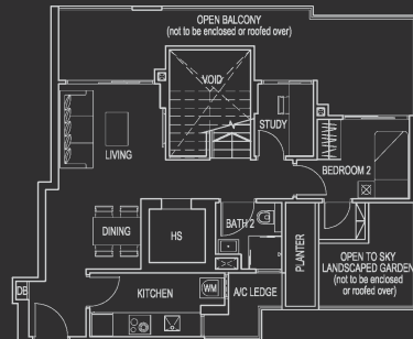
LOWER STOREY
