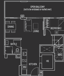
LOWER STOREY
