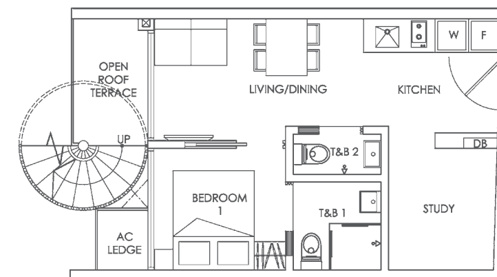
LOWER STOREY
