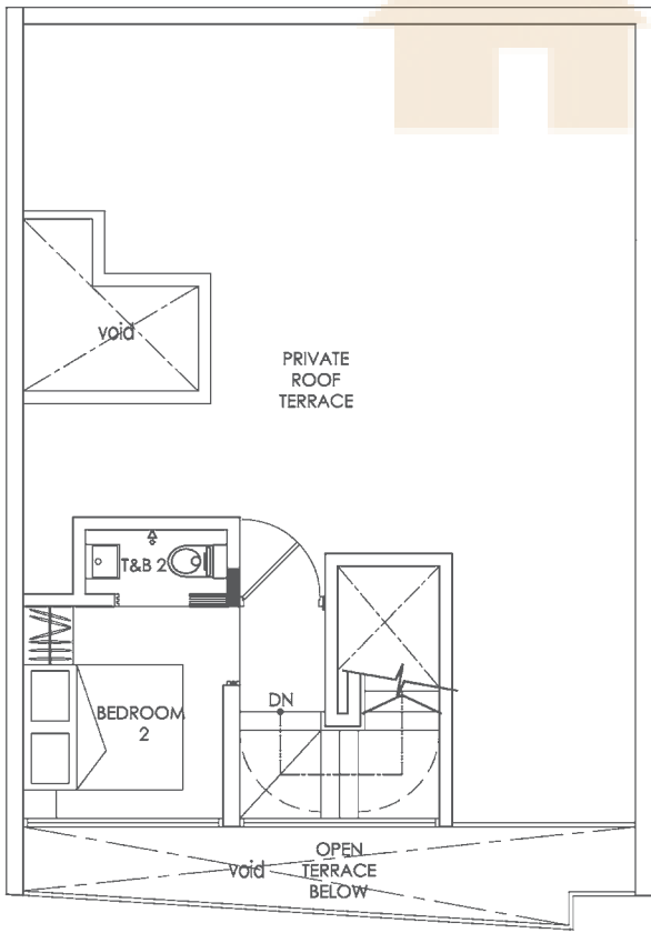
UPPER STOREY
