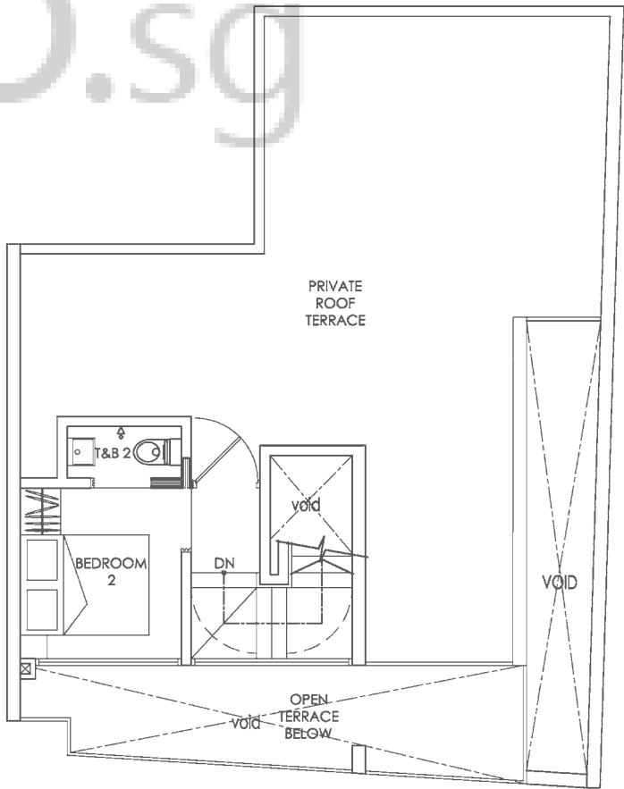
UPPER STOREY
