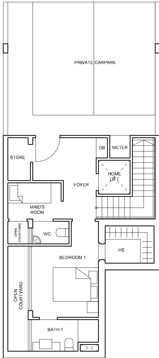
BASEMENT
