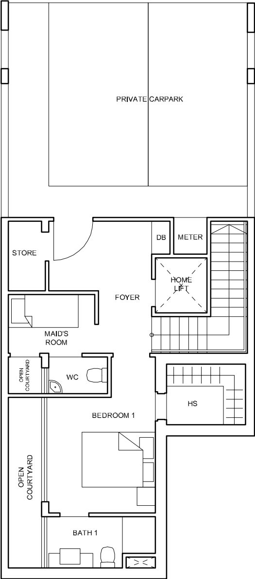
BASEMENT
