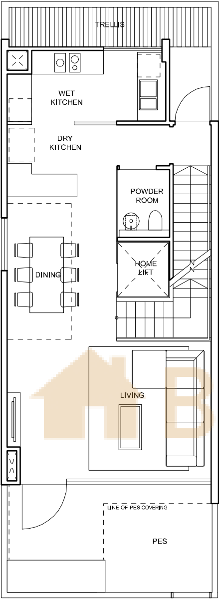
1ST STOREY
