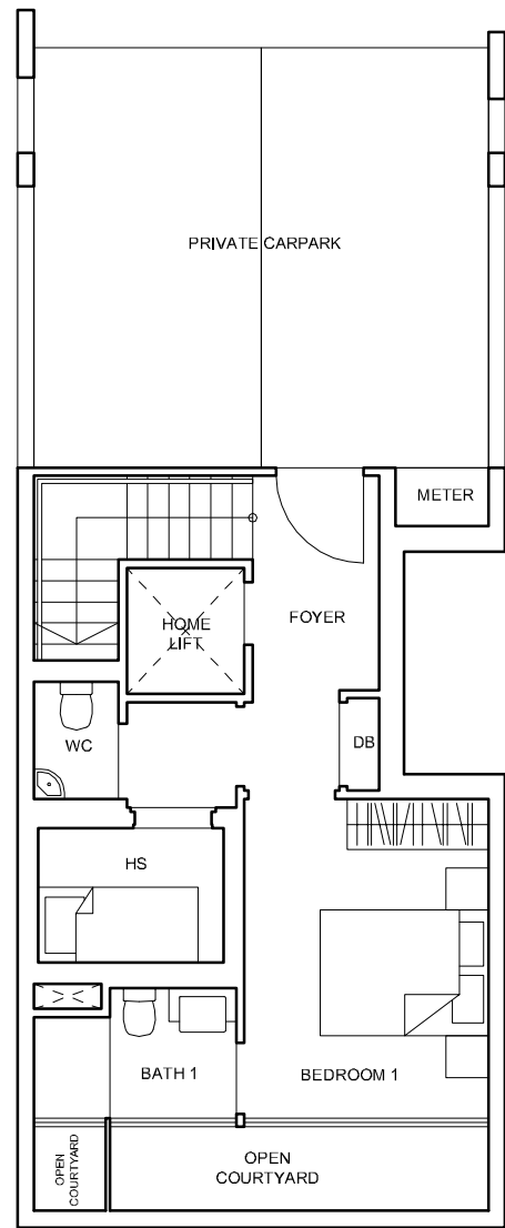
BASEMENT
