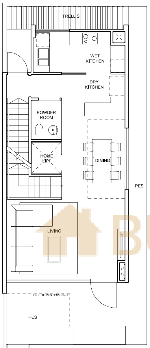
1ST STOREY
