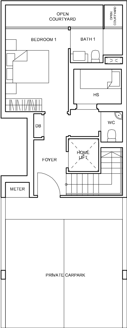
BASEMENT
