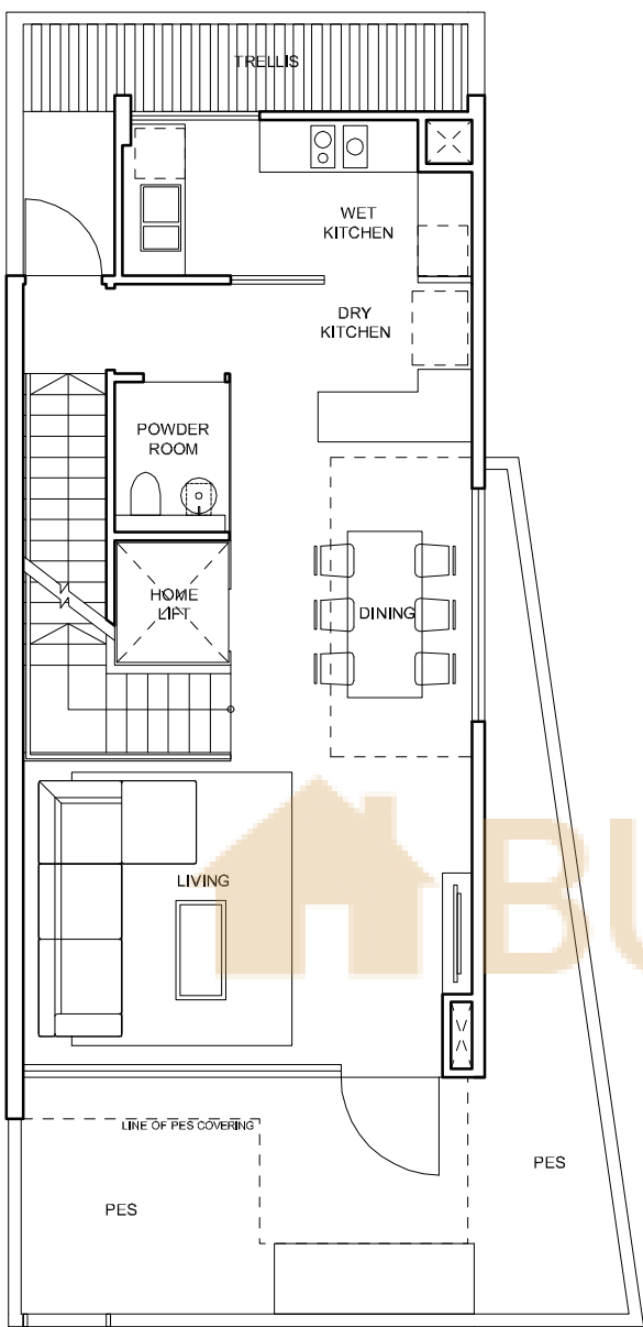
1ST STOREY
