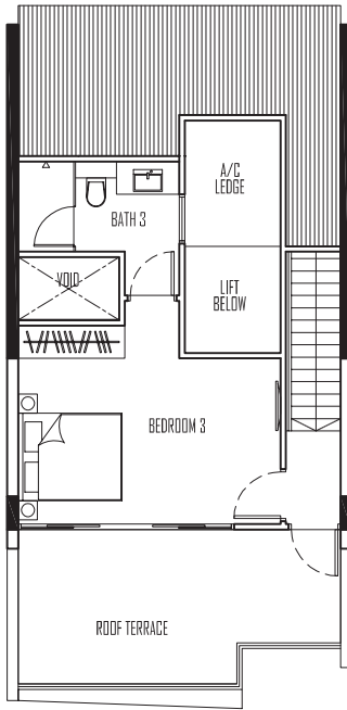
ATTIC
