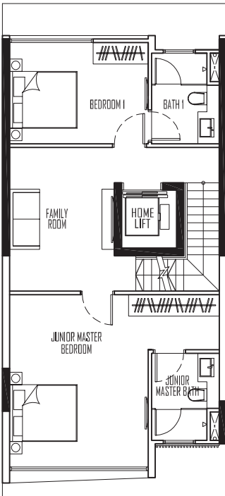
2ND STOREY
