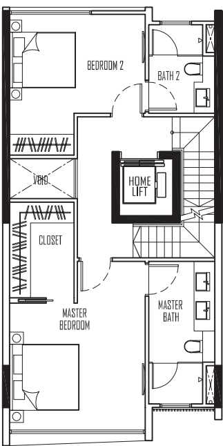
3RD STOREY
