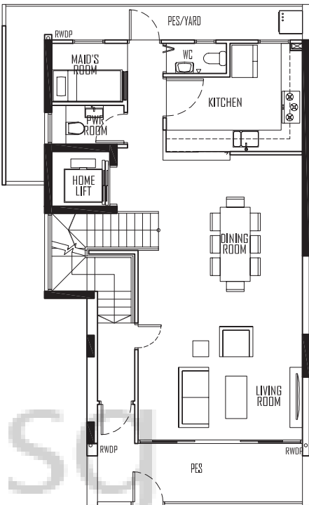
1ST STOREY
