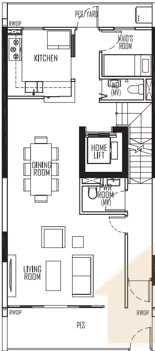
1ST STOREY
