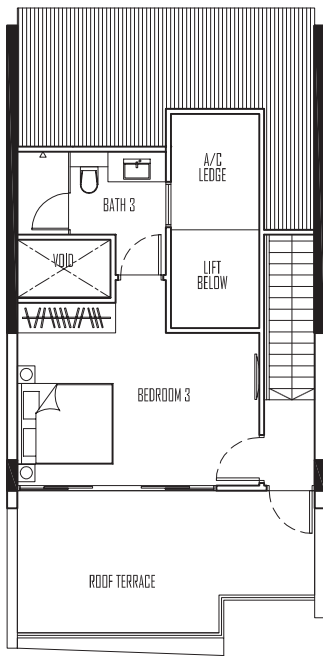
ATTIC
