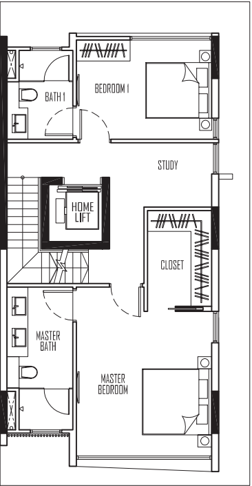
2ND STOREY
