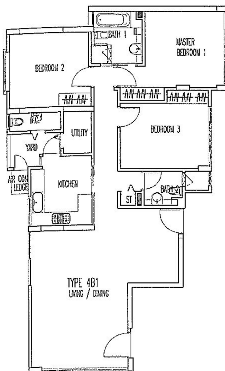
TYPE 4B1 (2ND – 3RD STOREY) Area 128 sq m / 1,378 sq ft
