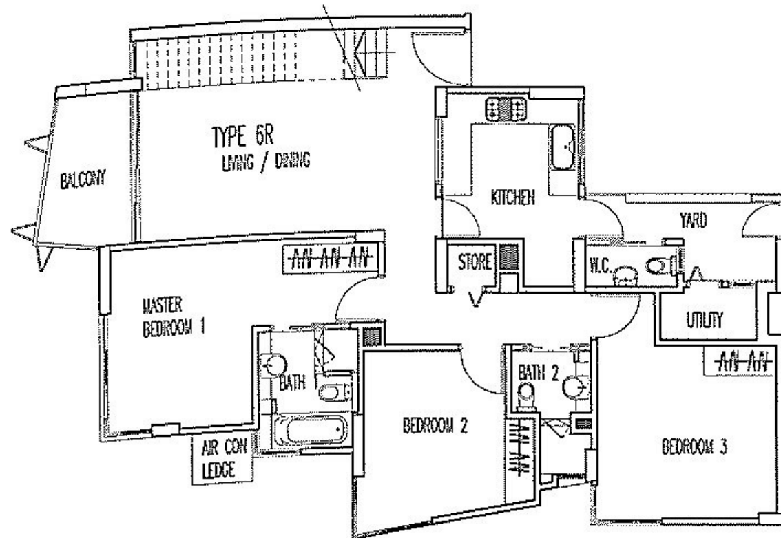
TYPE 6R (4TH STOREY) Area 158 sq m / 1,701 sq ft
