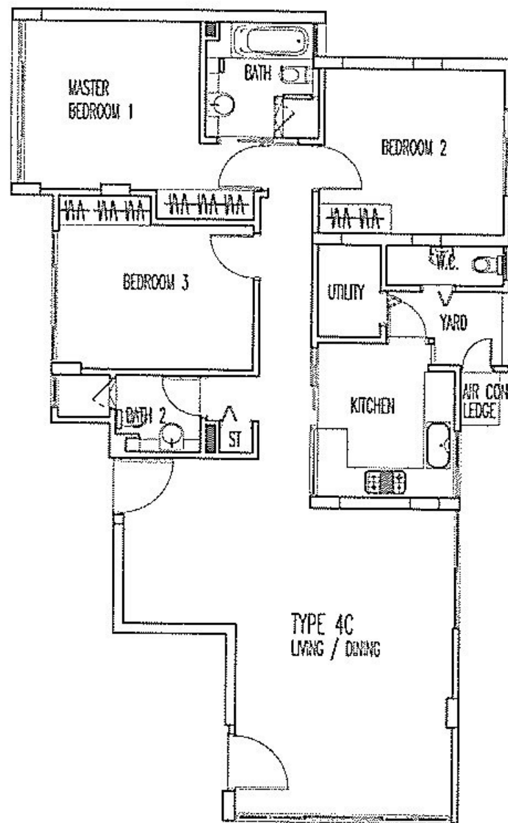
TYPE 4C (1ST STOREY) Area 128 sq m / 1,378 sq ft
