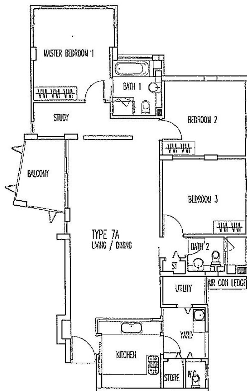
TYPE 7A (4TH STOREY) Area 138 sq m / 1,485 sq ft
