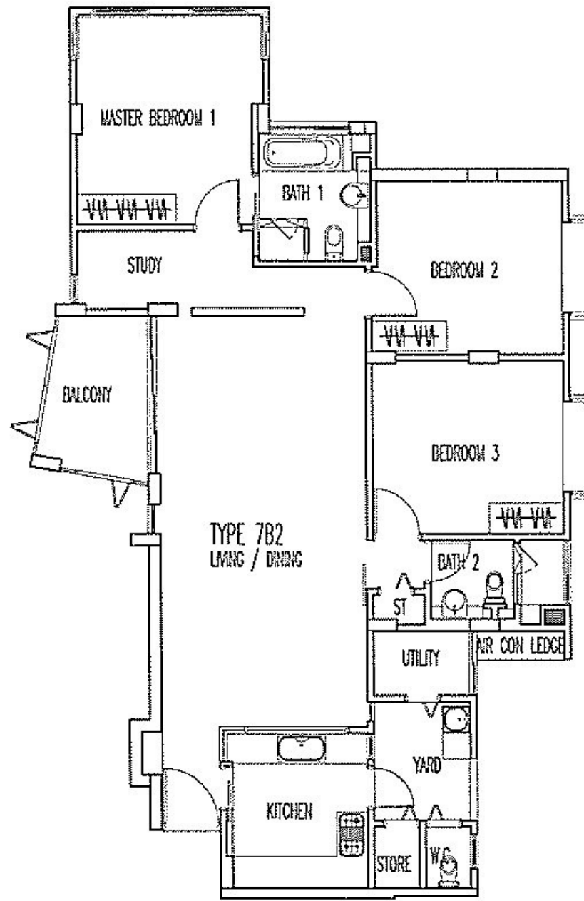
TYPE 7B2 (2ND – 3RD STOREY) Area 139 sq m / 1,496 sq ft
