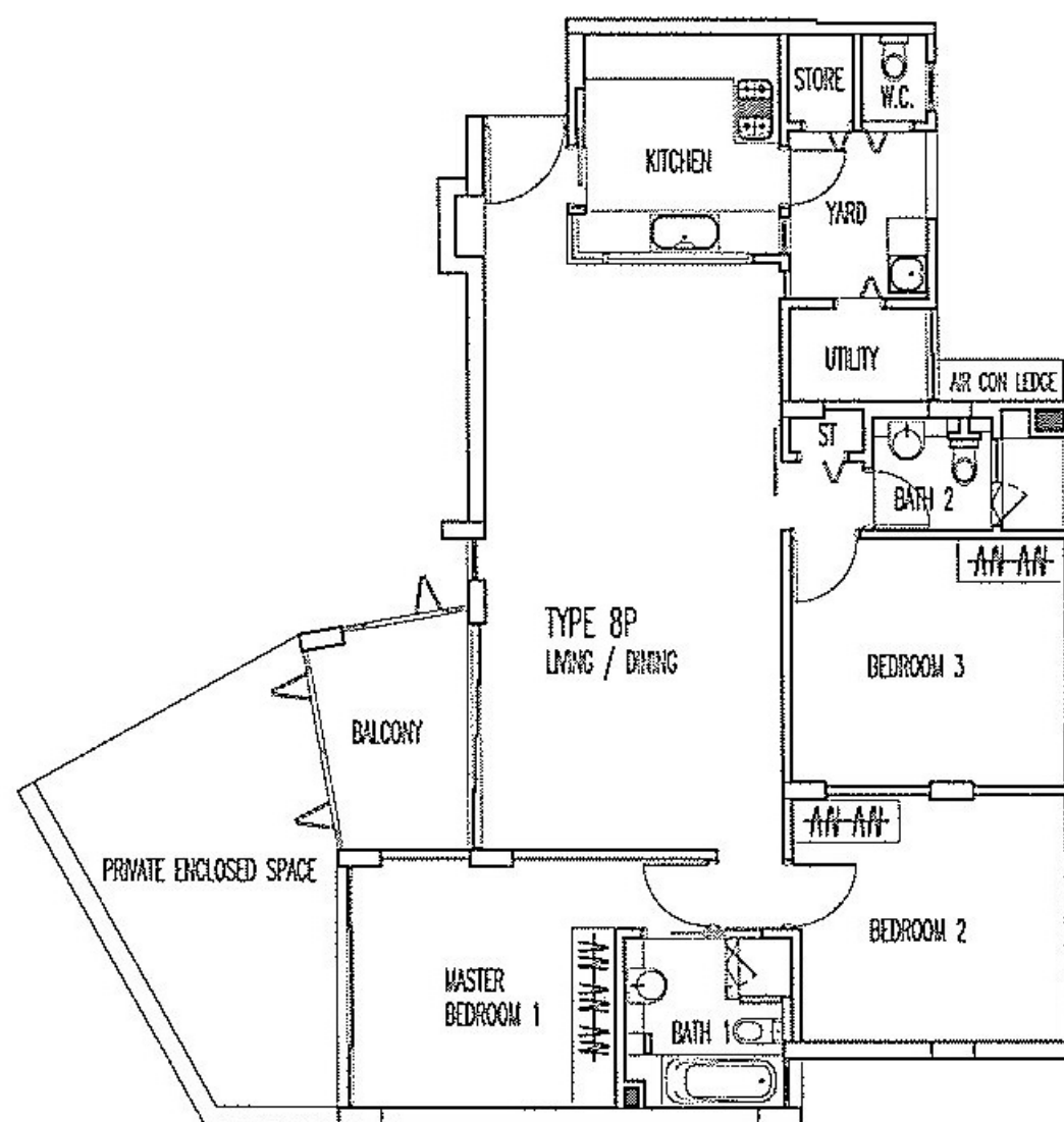
TYPE 8P (1ST STOREY) Area 150 sq m / 1,615 sq ft
