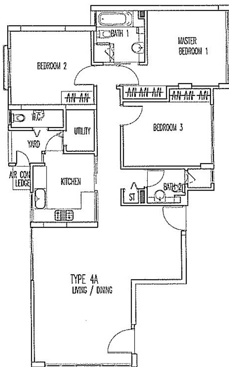
TYPE 4A (4TH STOREY) Area 128 sq m / 1,378 sq ft
