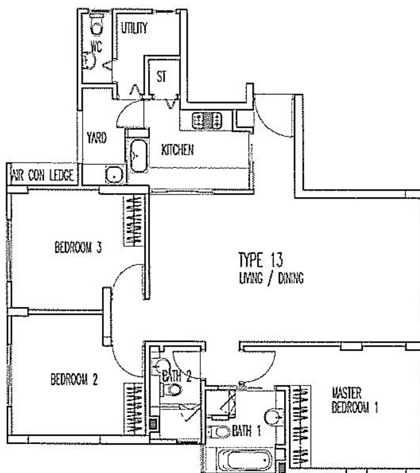
TYPE 13 (1ST STOREY) Area 119 sq m / 1,281 sq ft
