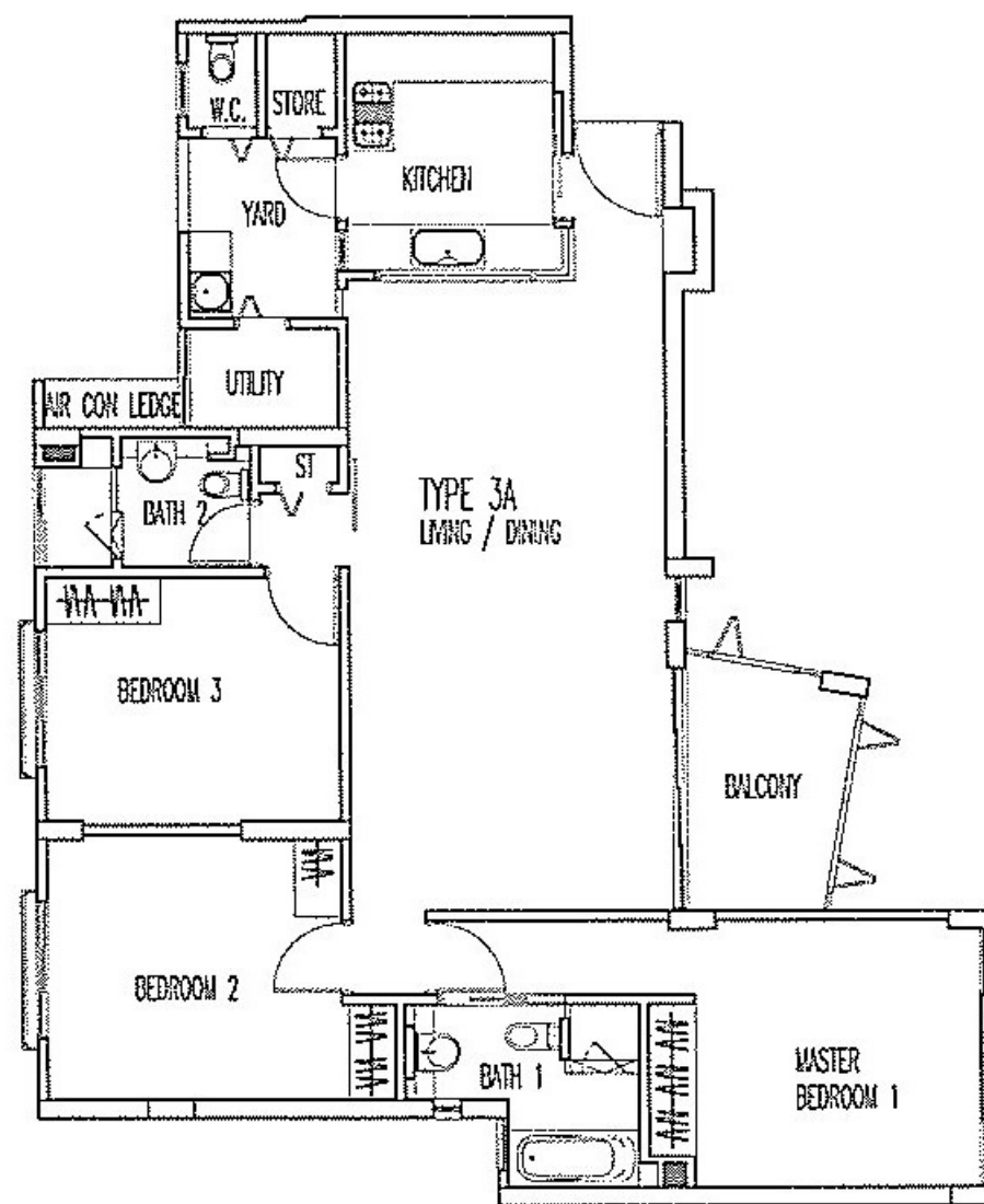
TYPE 3A (4TH STOREY) Area 134 sq m / 1,442 sq ft
