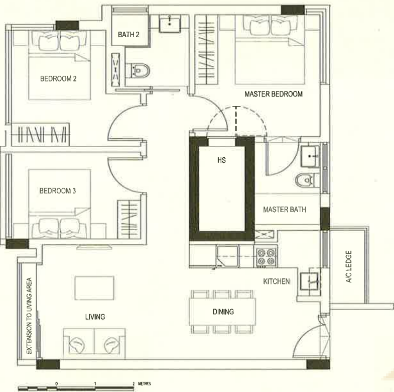
#02-06 (75 sqm)
