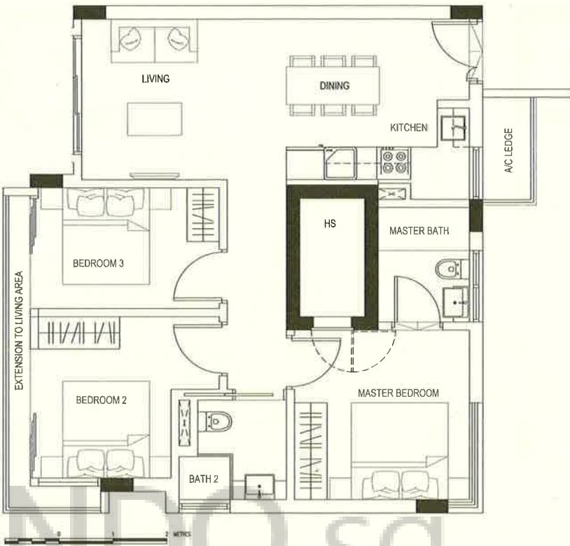
#02-05 (77 sqm)
