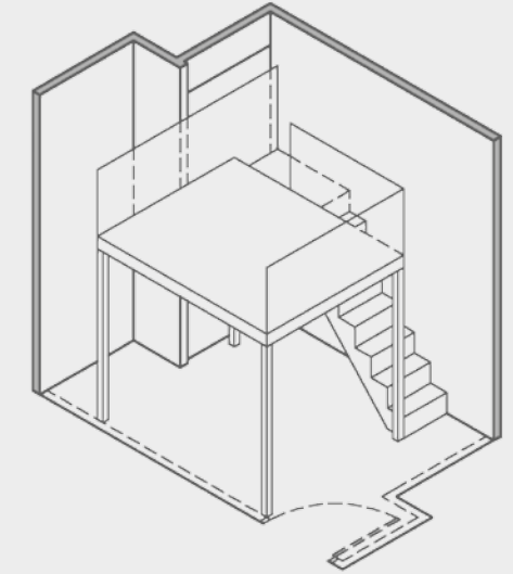
Suggested Furniture Loft - Isometric View (Only applicable to Master Bedroom with maximum area of 5 sqm)
