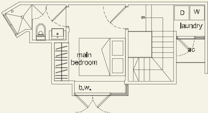
UPPER PENTHOUSE
