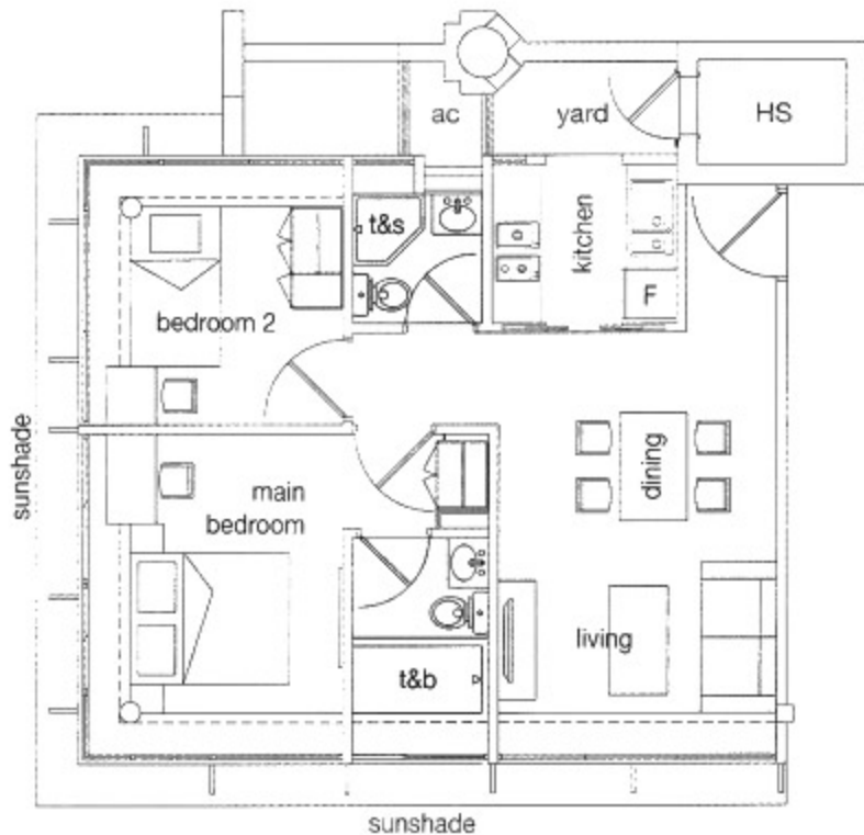
TYPE F # 05-01 (66 sqm / 710 sqft)
