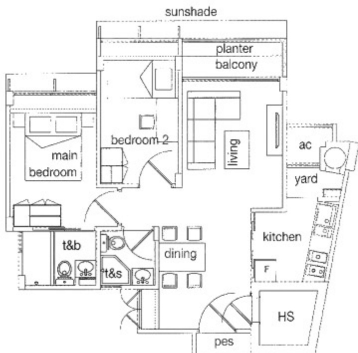
TYPE C # 02-03 | # 03-03 | # 04-03 (65 sqm / 700 sqft)
