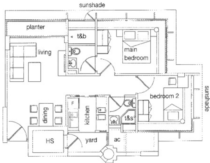
TYPE D # 02-04 | # 03-04 | # 04-04 (70 sqm / 753 sqft)
