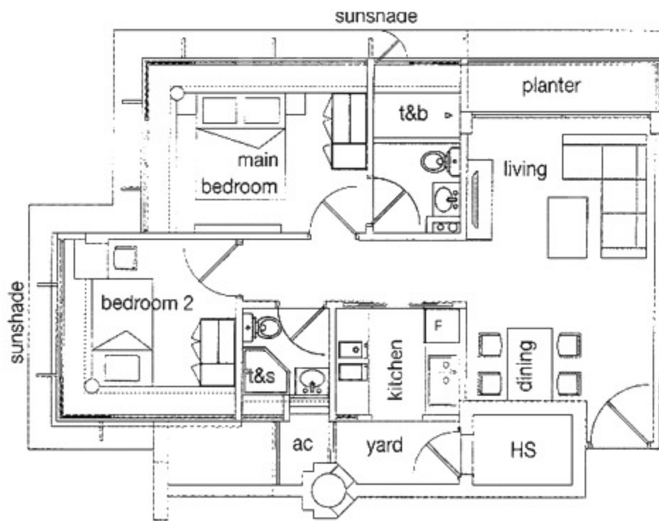
TYPE B # 02-02 | # 03-02 | # 04-02 (70 sqm / 753 sqft)
