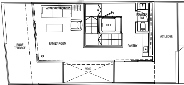
Attic Plan
