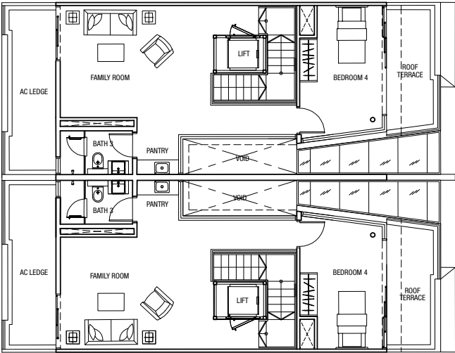
Attic Plan
