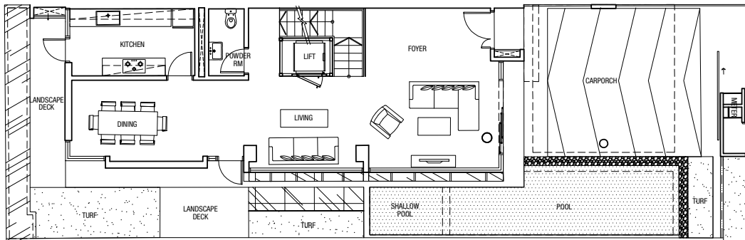
Level 1 Plan
