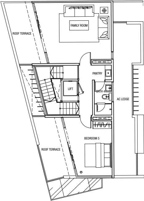
Attic Plan
