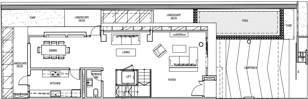
Level 1 Plan
