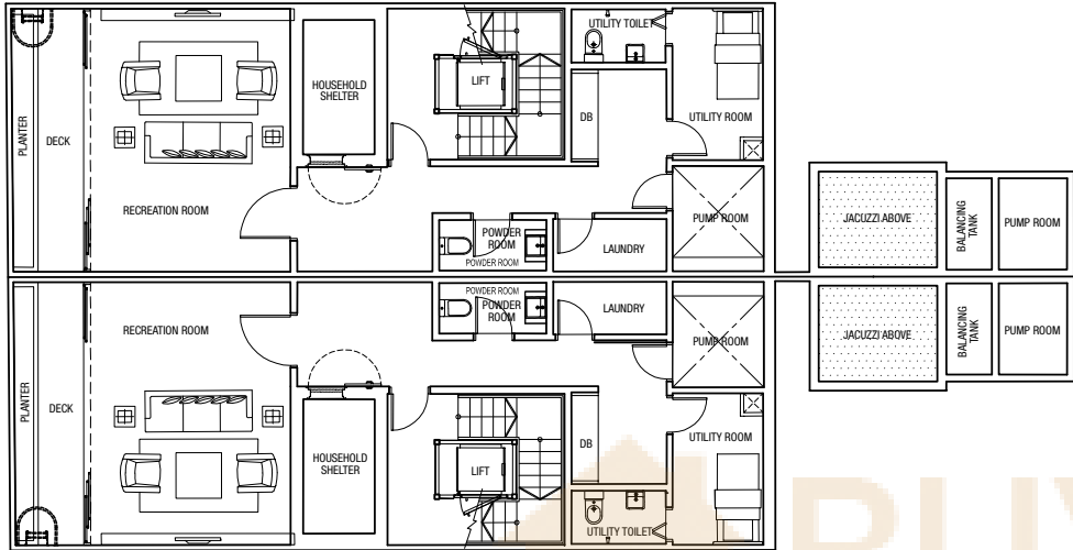
Basement Plan
