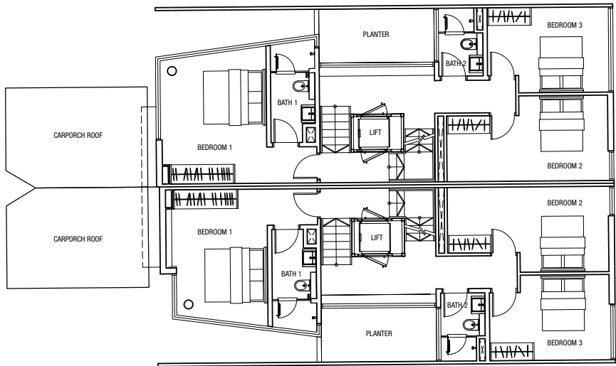
Level 3 Plan
