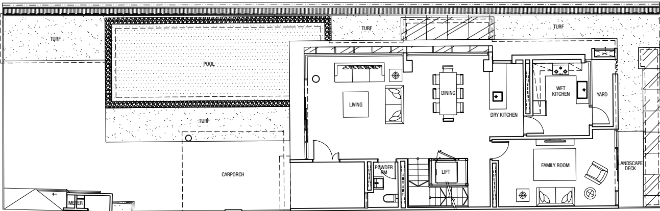
Level 1 Plan
