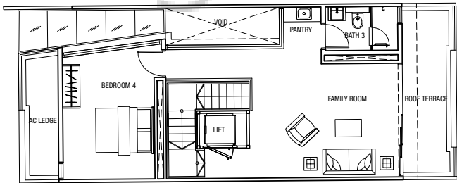
Attic Plan
