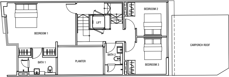
Level 3 Plan
