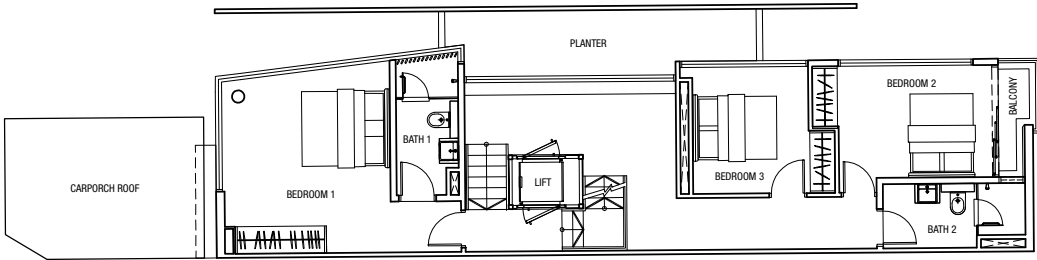
Level 2 Plan
