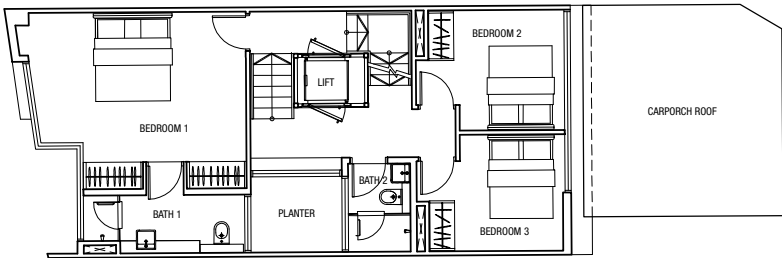
Level 2 Plan
