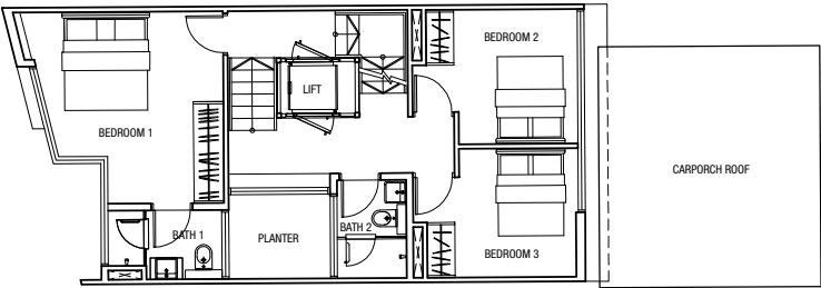
Level 2 Plan
