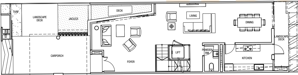
Level 1 Plan
