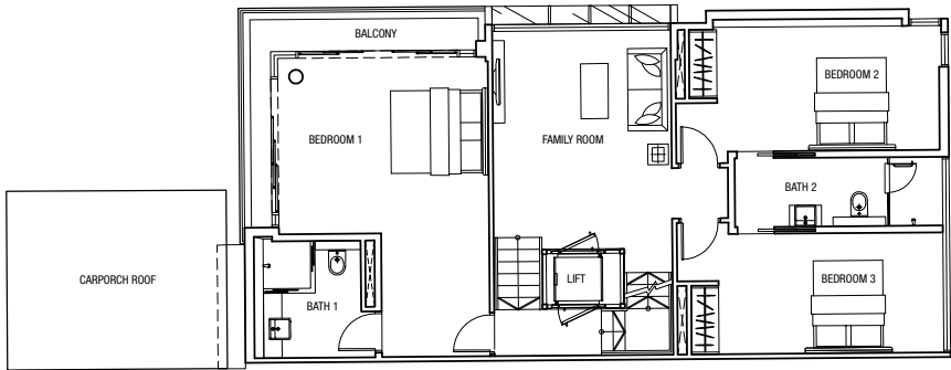
Level 3 Plan
