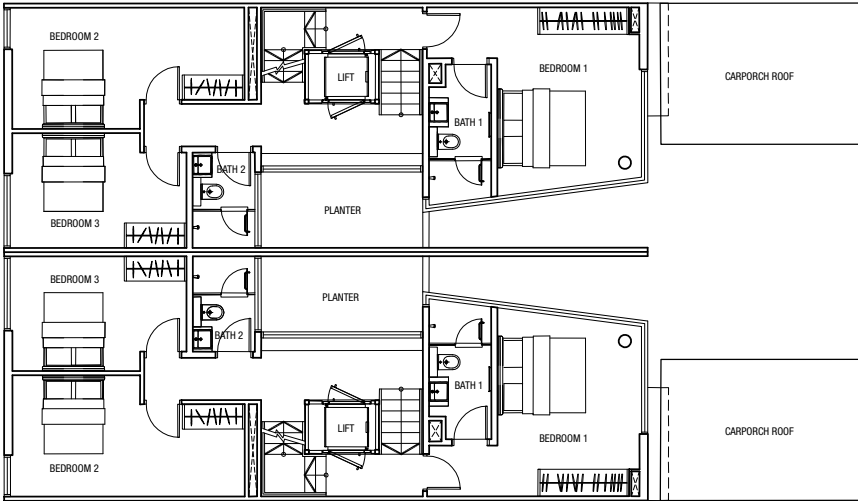
Level 2 Plan
