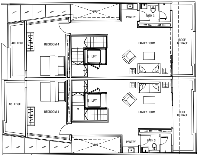
Attic Plan
