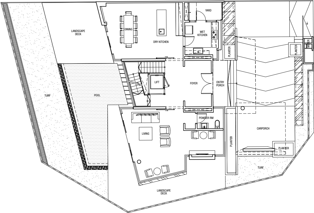
Level 1 Plan
