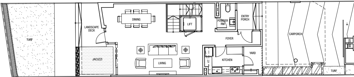
Level 1 Plan
