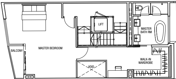
Level 3 Plan
