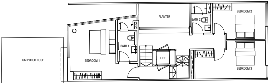
Level 2 Plan
