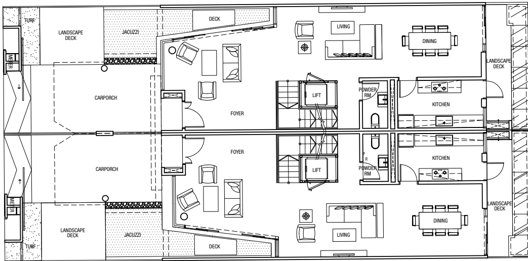
Level 1 Plan
