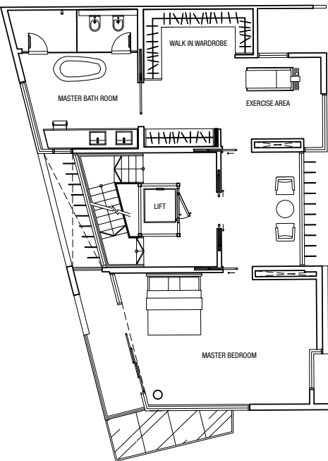
Level 3 Plan
