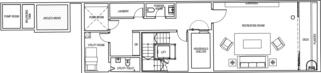
Basement Plan
