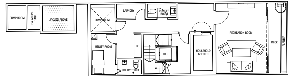
Basement Plan
