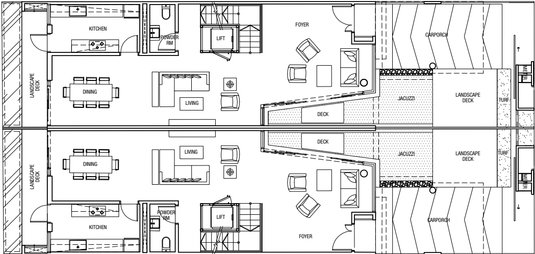
Level 1 Plan
