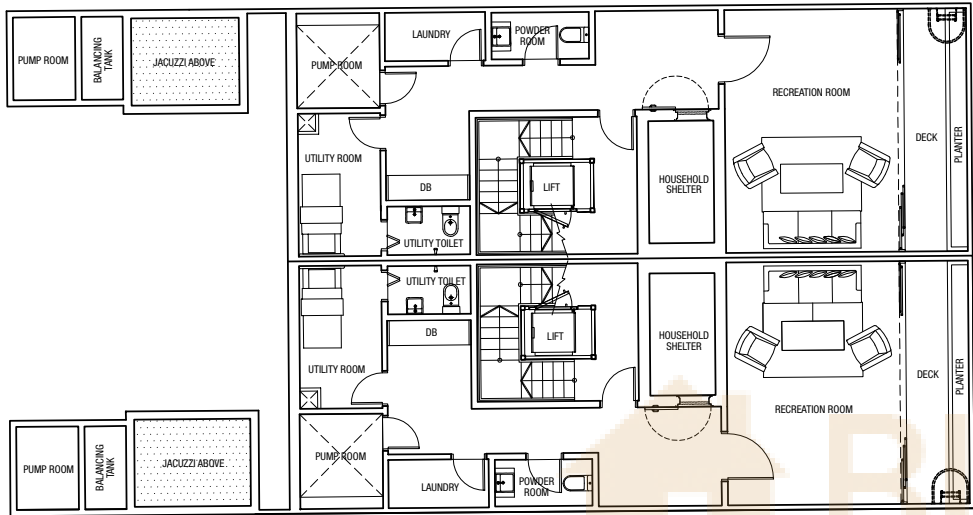
Basement Plan
