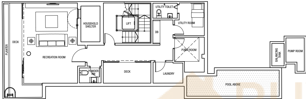
Basement Plan
