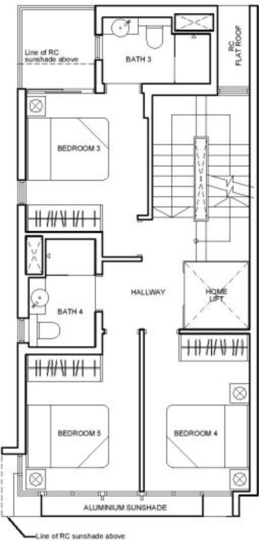
3RD STOREY
