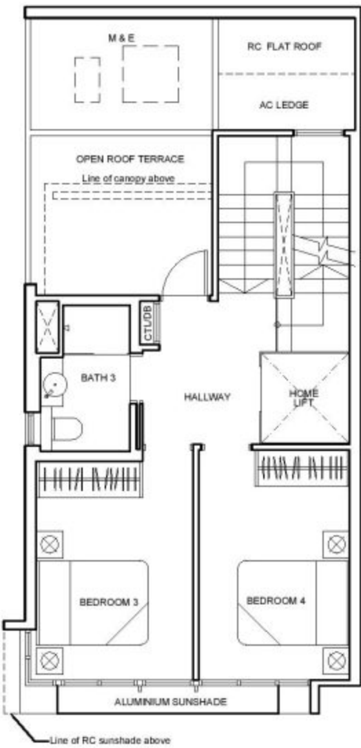
ATTIC
