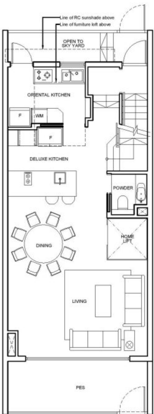
1ST STOREY
