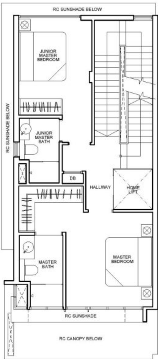
2ND STOREY
