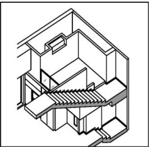
LOFT - ISOMETRIC VIEW
