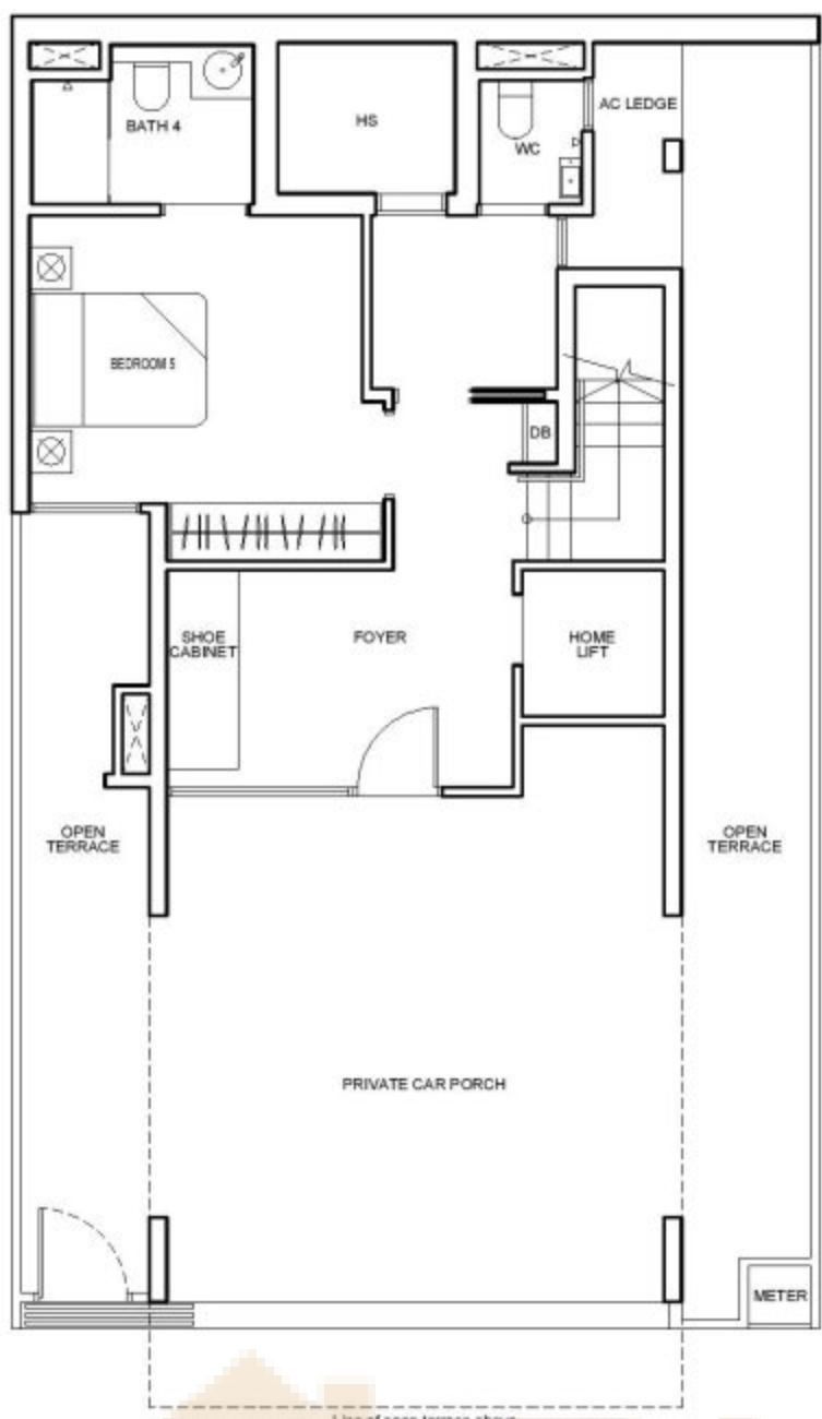
1ST STOREY
