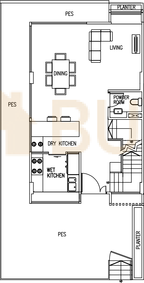
1st STOREY
