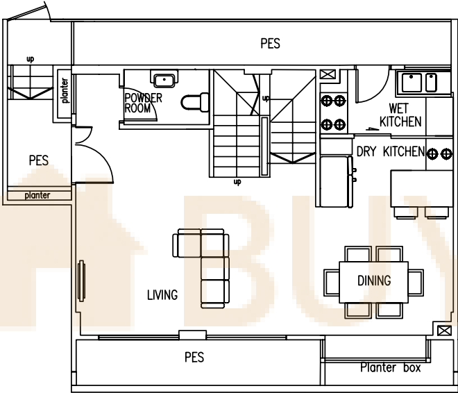
1st STOREY
