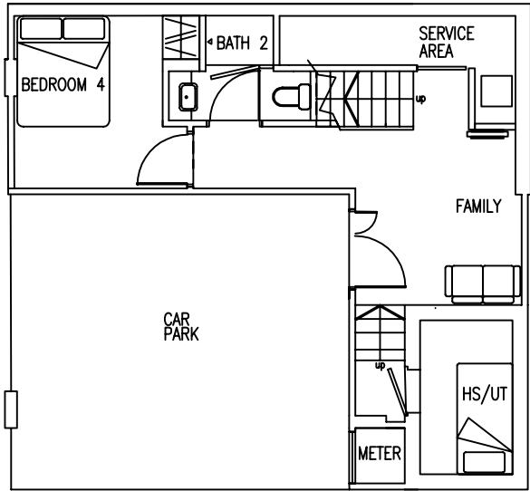
BASEMENT
