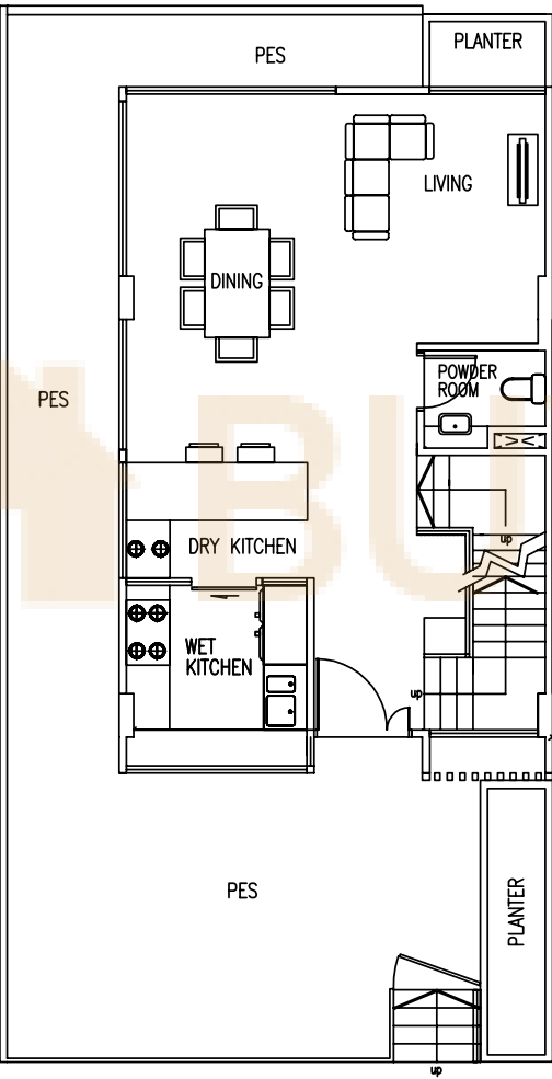
1st STOREY
