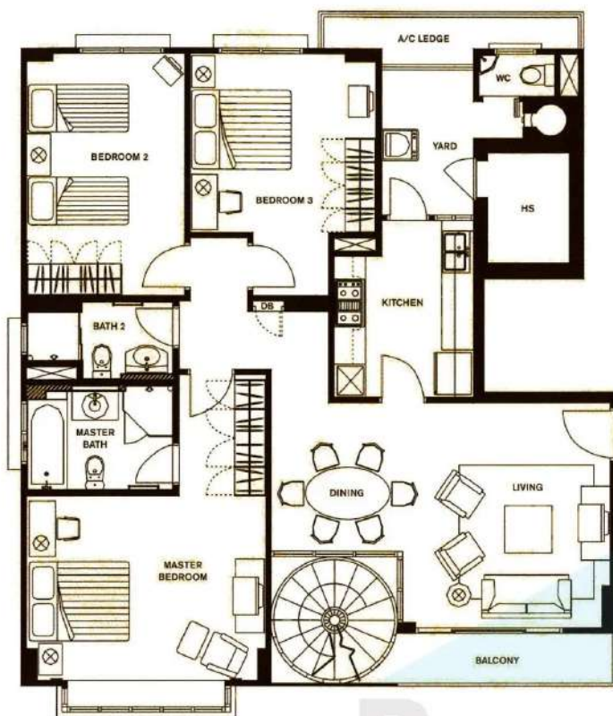
lower storey
