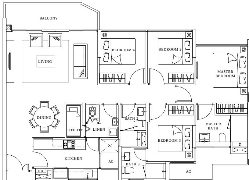
TYPE D1b 124 sq.m. / 1335 sq.ft. #02-08 to #17-08
