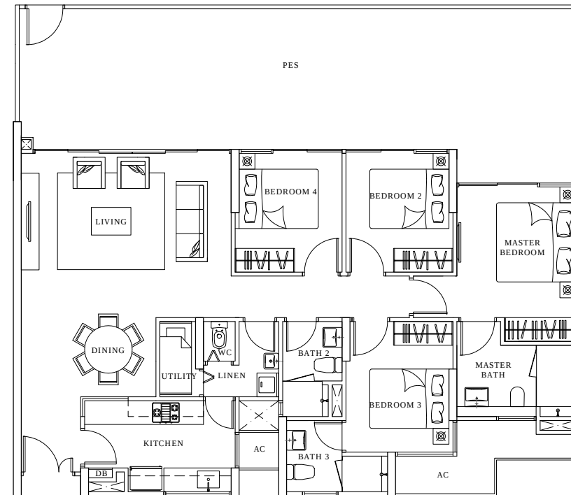
TYPE D1p 171 sq.m. / 1841 sq.ft. #01-08
