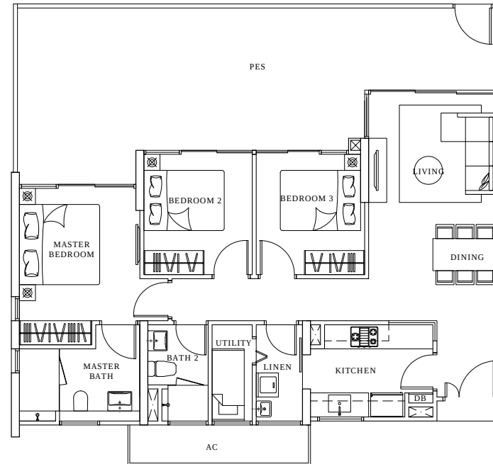
TYPE B1p 130 sq.m. / 1399 sq.ft. #01-17
