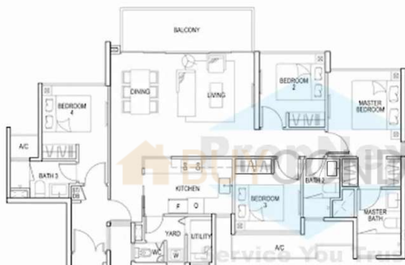
TYPE C3b1 4 BEDROOM (DUAL KEY) SFA = 126 sqm
