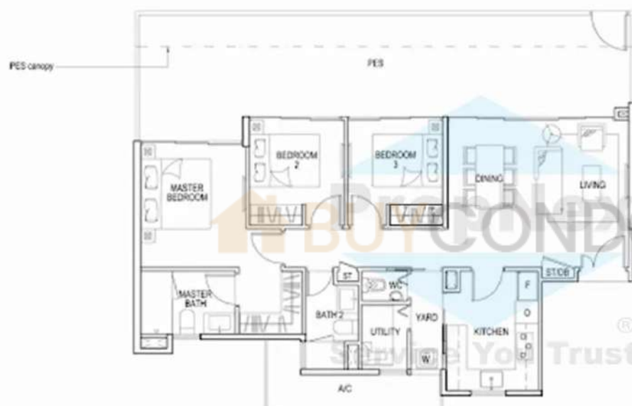
TYPE B5P1 3 BEDROOM SFA = 140 sqm #01-20 #01-31(minor)
