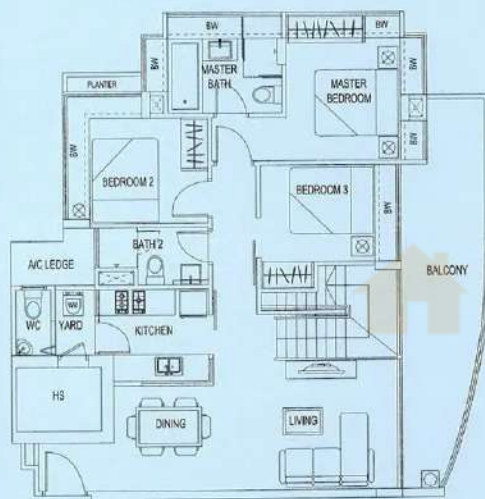
Lower Storey
