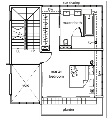
2 nd Storey (87 sqm)
