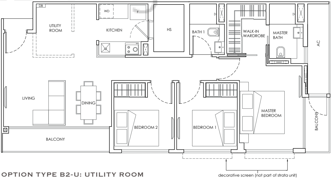
OPTION TYPE B2-U: UTILITY ROOM
