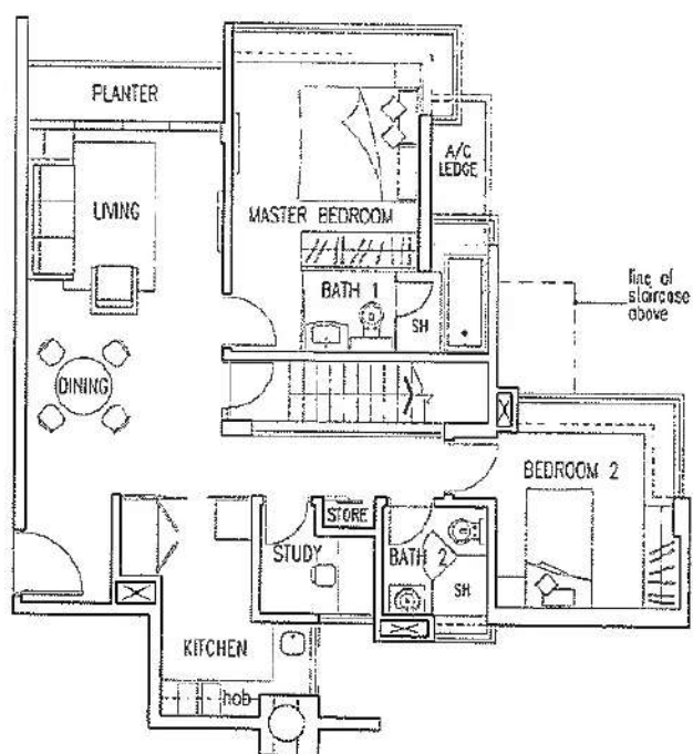
LOWER STOREY
