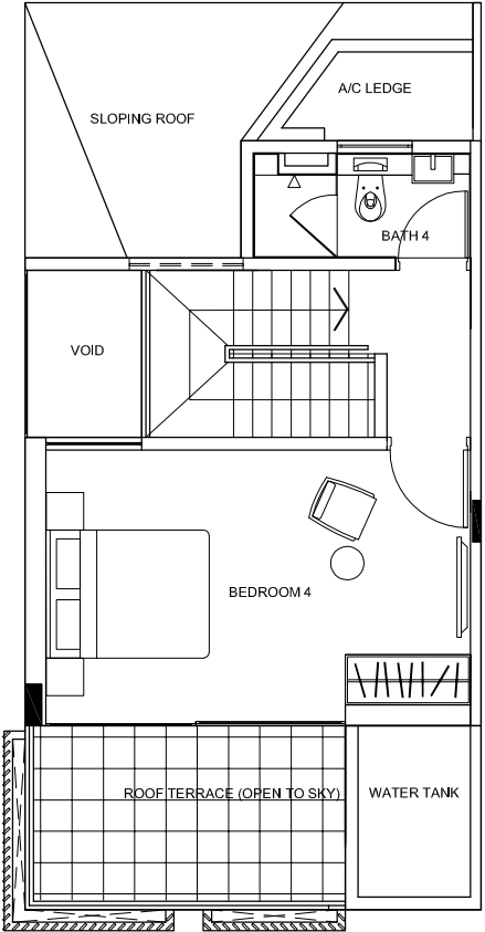
ATTIC
