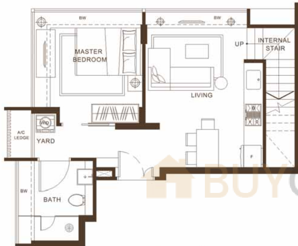
Lower Storey
