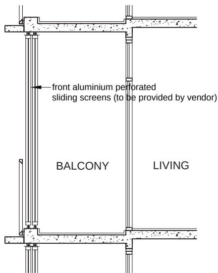
SLIDING BALCONY SCREEN - SECTION
