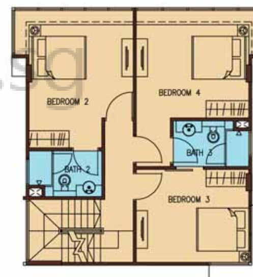
ATTIC PLAN
