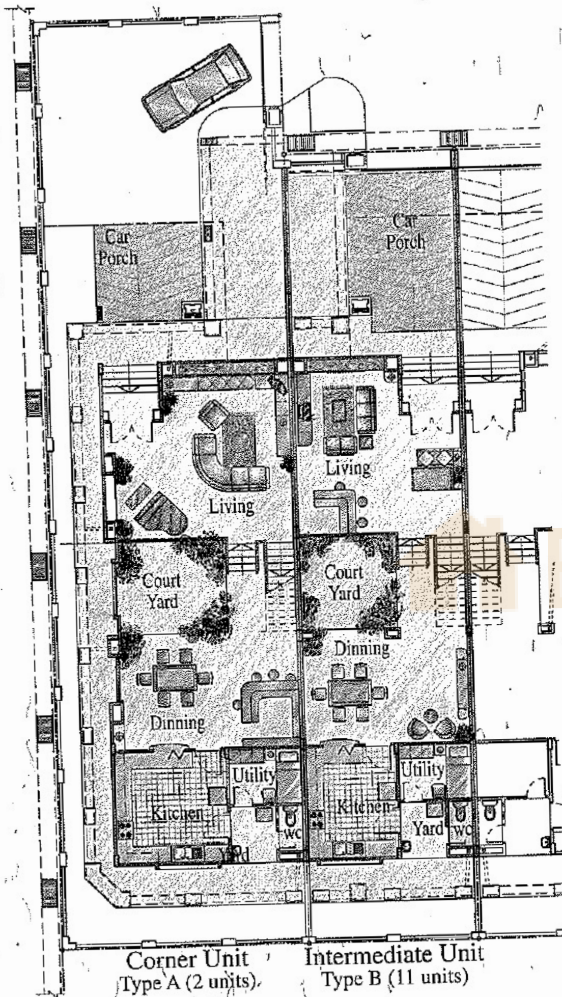
1st Storey Plan
