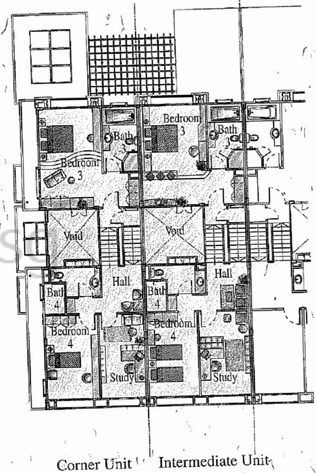
3rd Storey Plan
