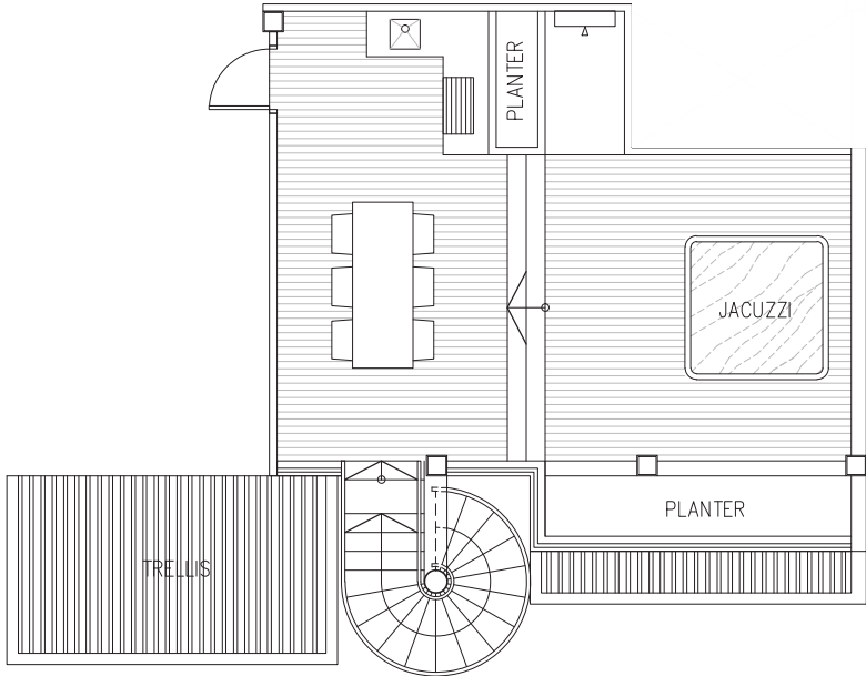
Roof Terrace
