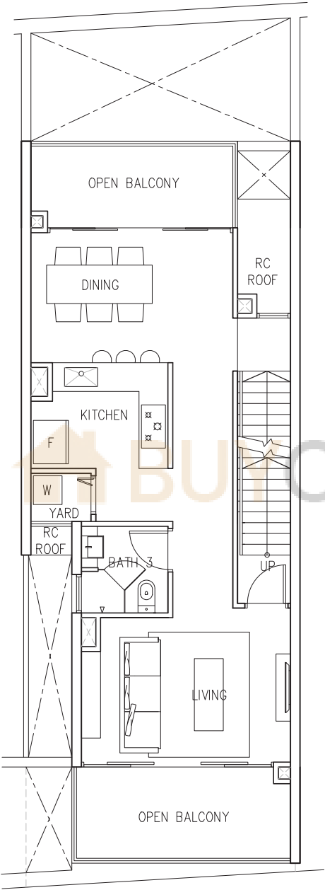
2ND STOREY
