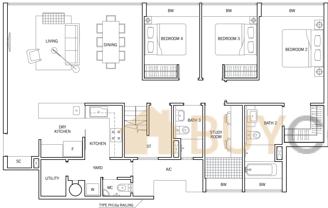
LOWER FLOOR
