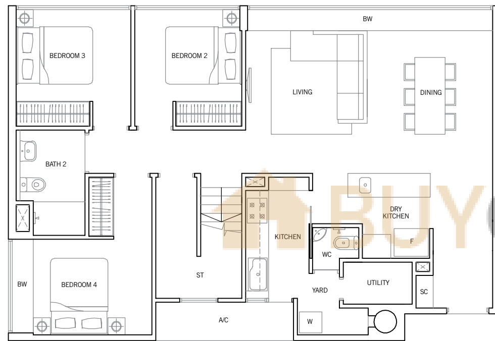
LOWER FLOOR
