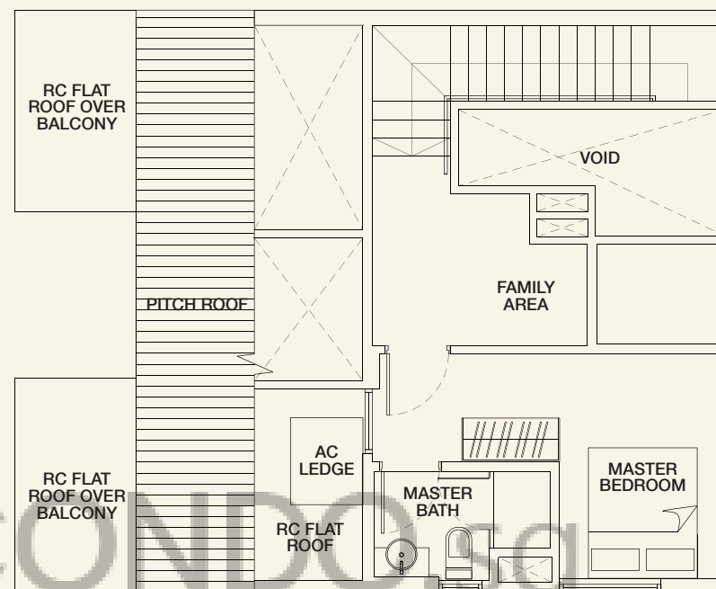
UPPER LEVEL
