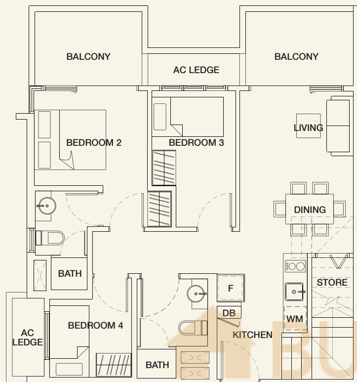
LOWER LEVEL
