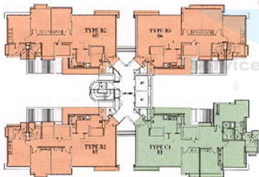
5TH, 8TH, 11TH, 14TH & 17TH STOREY PLAN
