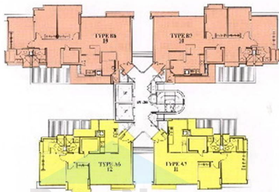
4TH, 7TH, 10TH, 13TH, 16TH & 19TH STOREY PLAN
