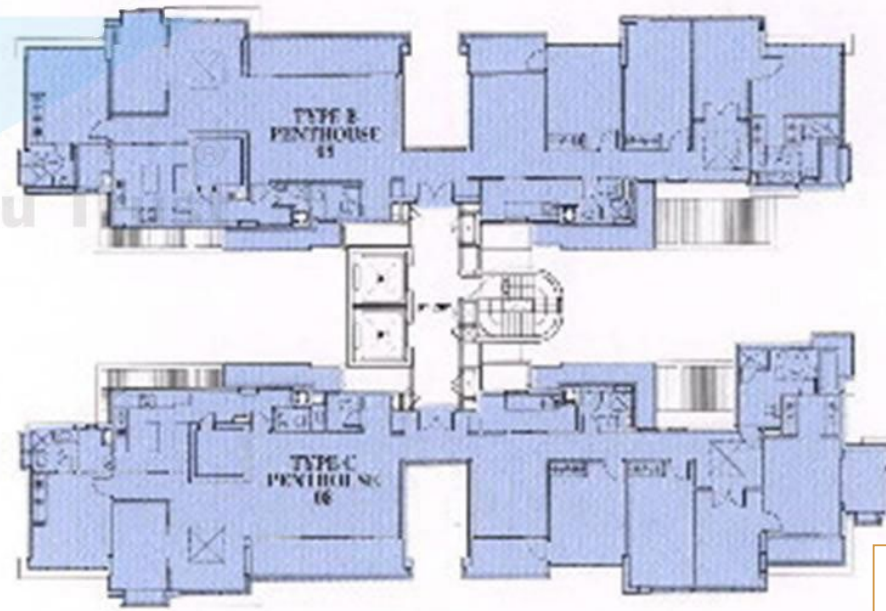
20TH STOREY PLAN
