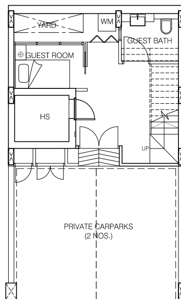
BASEMENT PLAN
