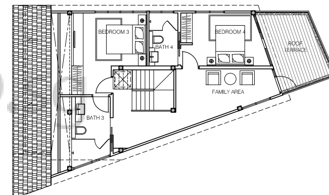
ATTIC PLAN
