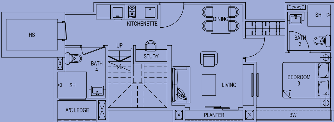
LOWER STOREY
