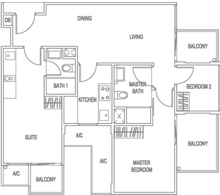
Type B5a #02-03 to #04-03 Area 85 sqm
