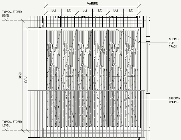
3 BALCONY / PES SCREEN - FRONT ELEVATION (External View)
