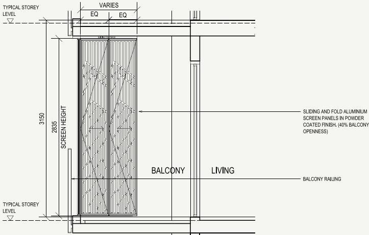
2 BALCONY / PES SCREEN - SECTION A-A (Internal View)
