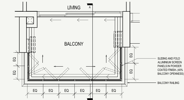
1 BALCONY / PES SCREEN - PLAN
