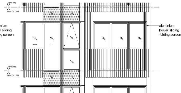
TYPICAL RETRACTABLE BALCONY SCREEN - ELEVATION (FULLY RETRACTED)
