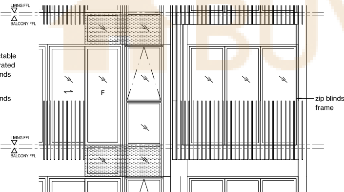
TYPICAL RETRACTABLE BALCONY SCREEN - ELEVATION (FULLY RETRACTED)
