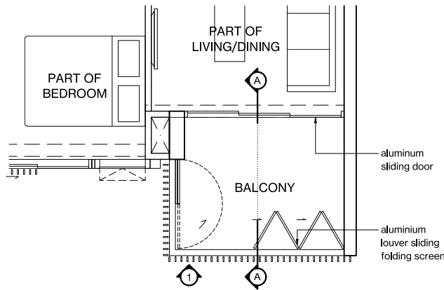
TYPICAL RETRACTABLE BALCONY SCREEN - PLAN
