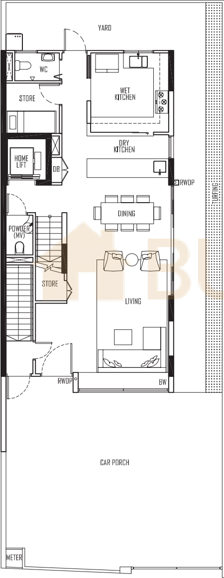
1ST STOREY PLAN
