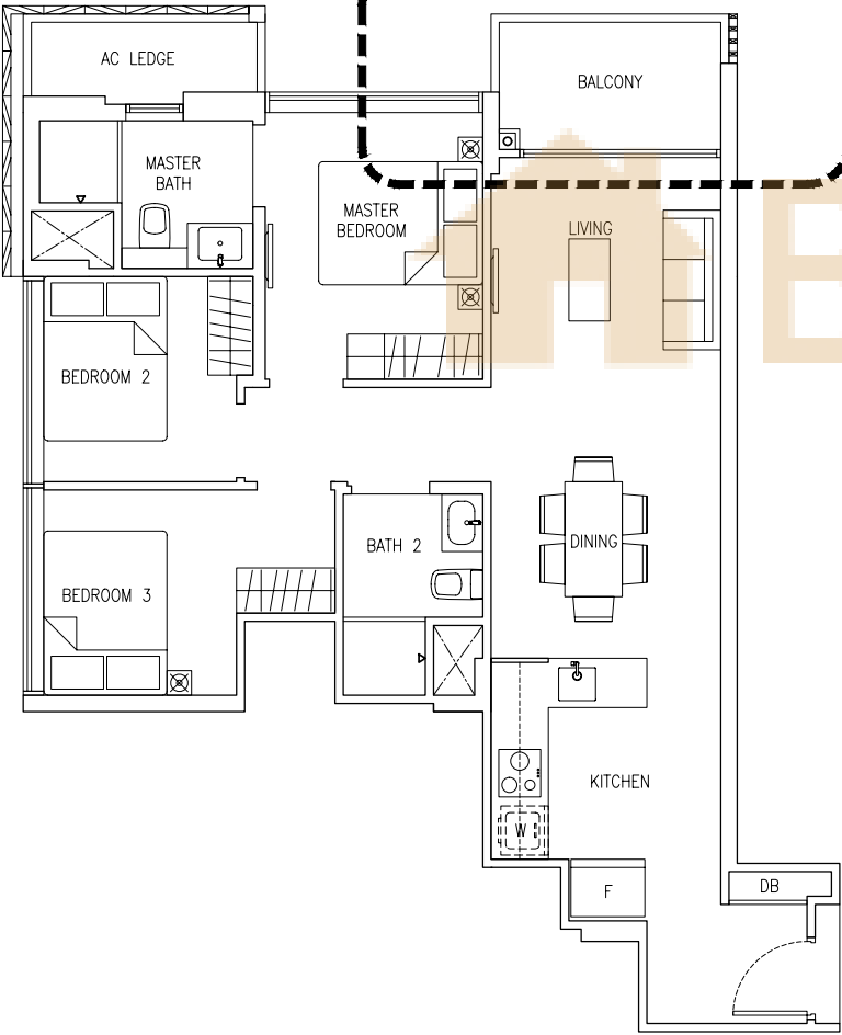
UNIT C1a #02 - 04 #04 - 04
