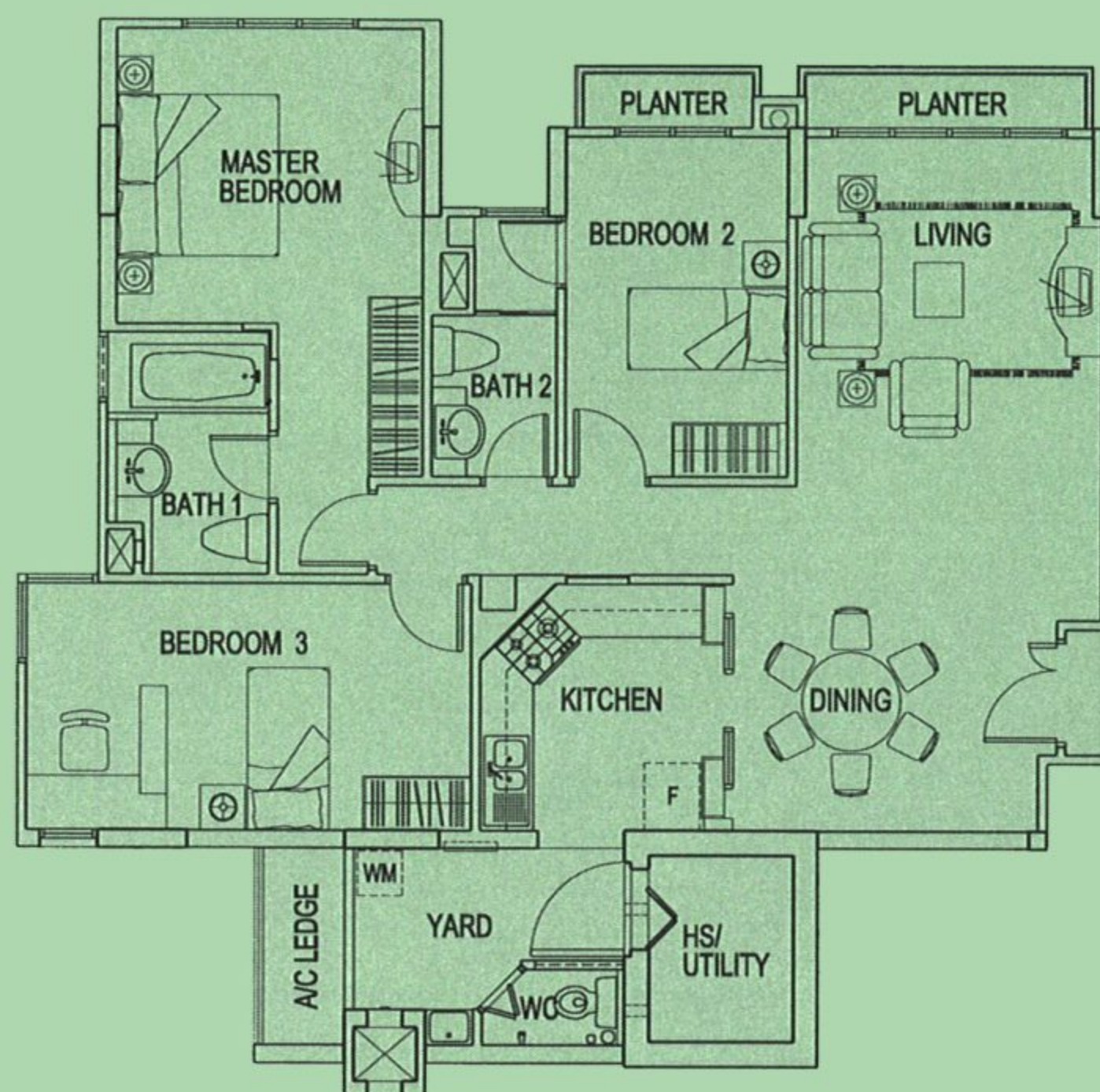
TYPE B 111 sqm (1195 sq ft)
