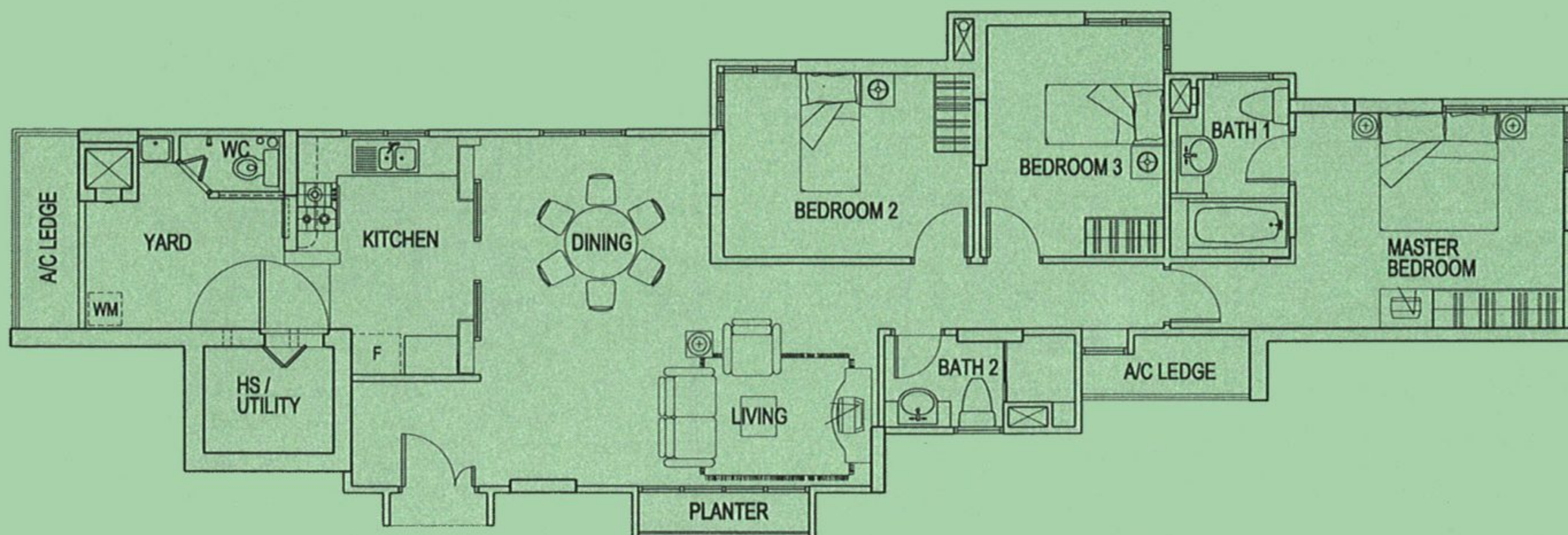
TYPE H 118 sqm (1270 sq ft) #03-15 to #12-15
