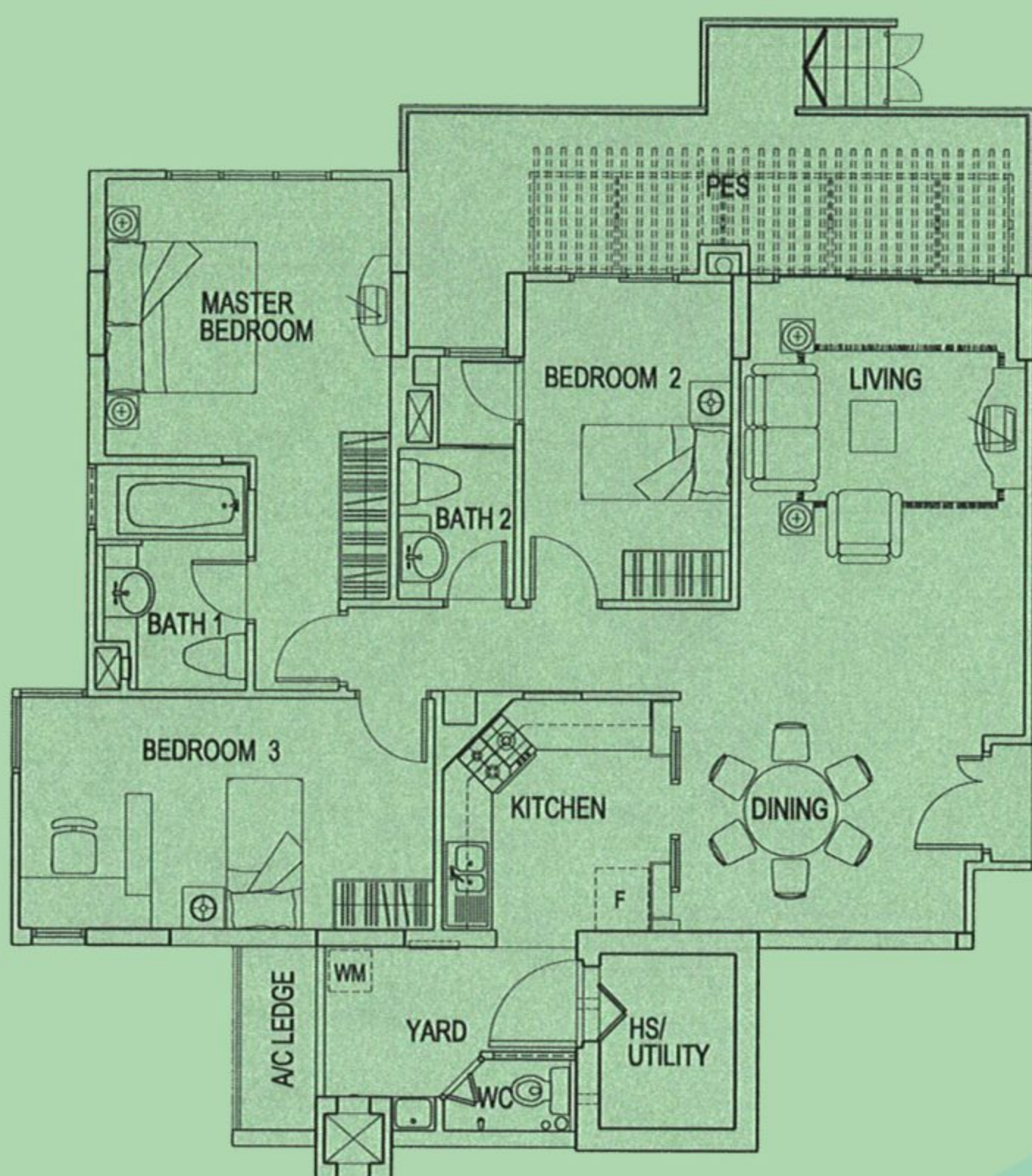
TYPE B (P) 126 sqm (1356 sq ft)
