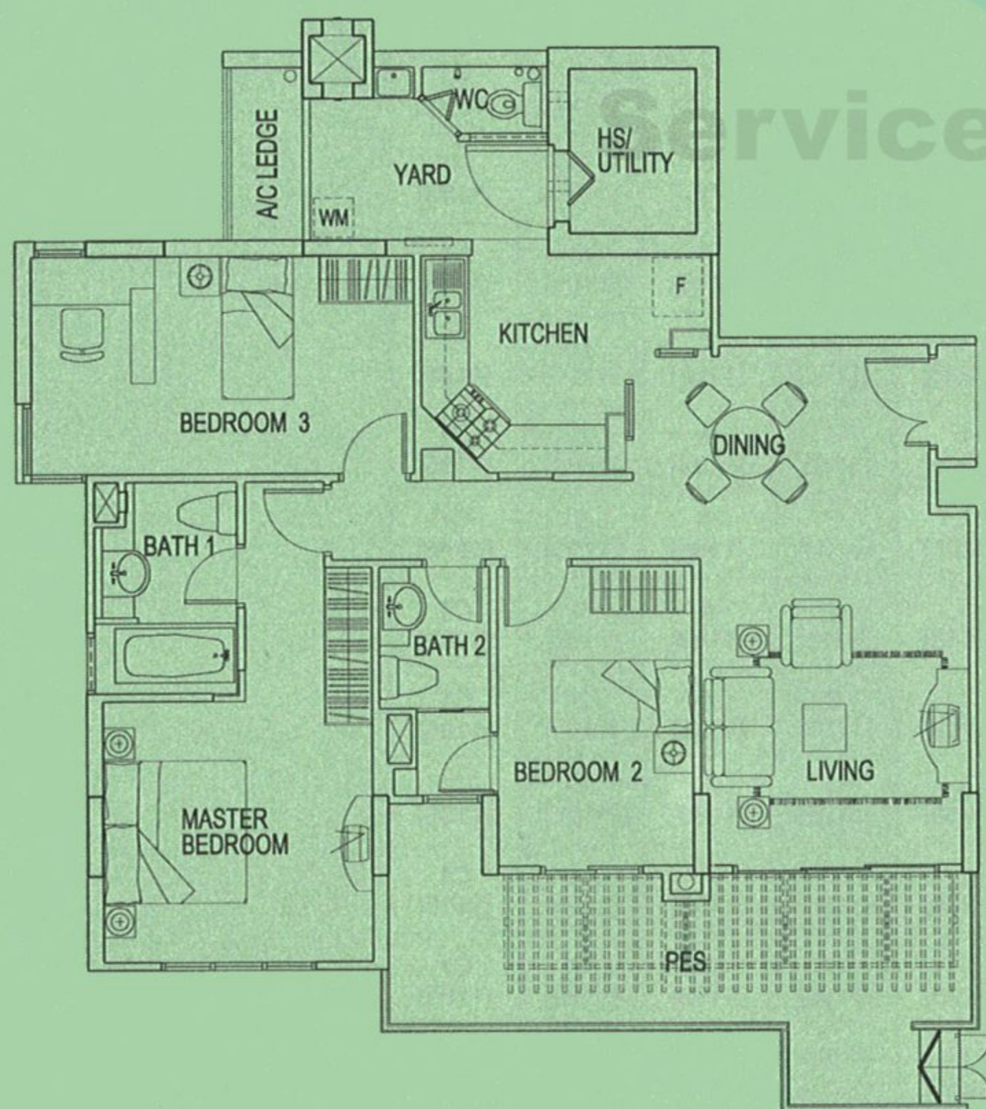
TYPE A1 (P) 122 sqm (1313 sq ft)
