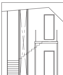
TYPE PH A – LOFT ELEVATION
