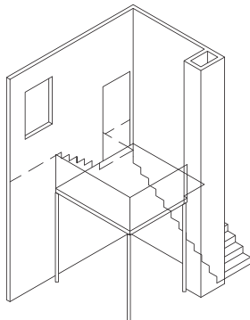
TYPE FM – LOFT ISOMETRIC VIEW
