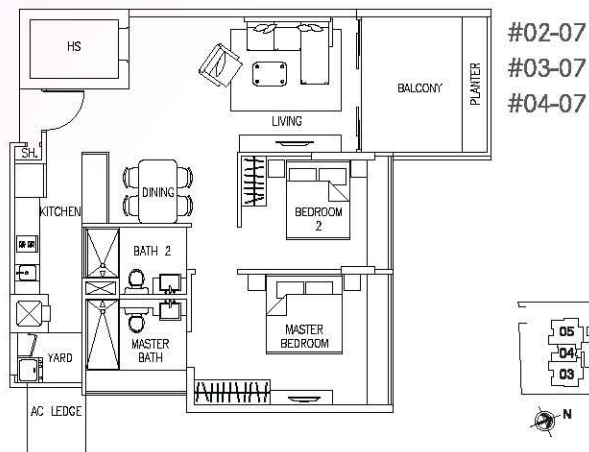
Type B1 (91 sq m / 980 sq ft)
