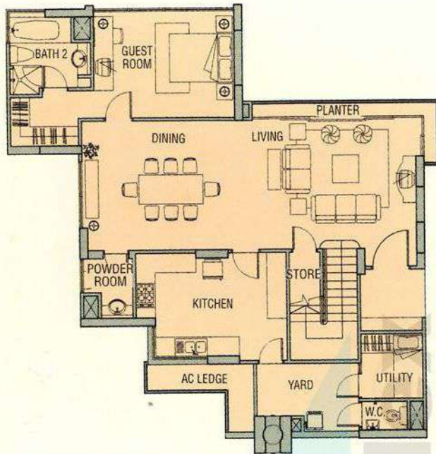
17th Storey – Lower Level
