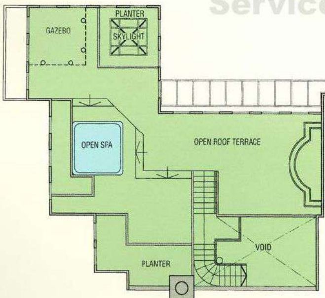
Roof Level – Roof Terrace
