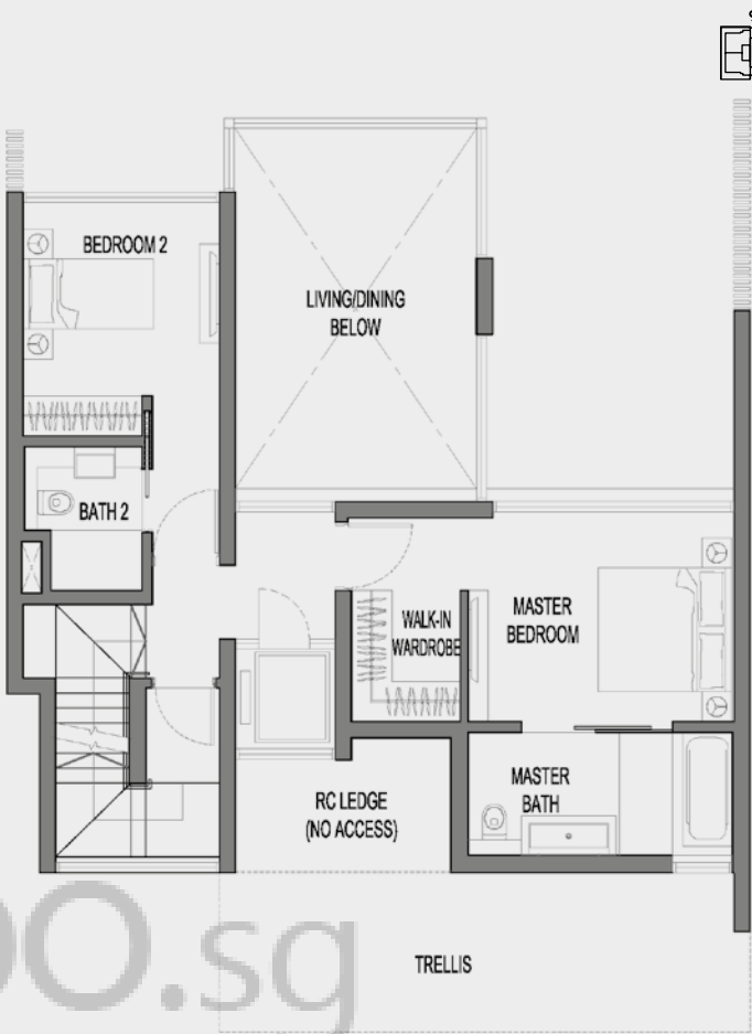
Level 2
