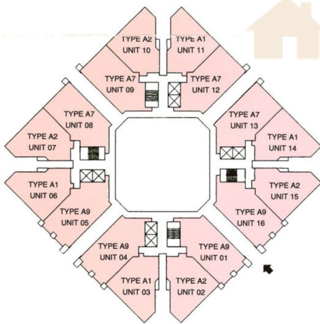
1ST STOREY (BLK 3)
